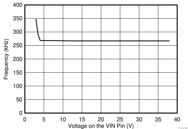
6-7. Minimum Switching Frequency for Quick Recovery from Frequency Foldback
