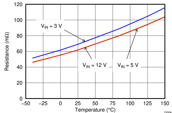
FIG 6-4. R_{DS(ON)} vs Temperature
