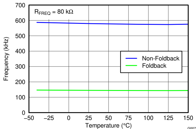
6-8. Nonfoldback Frequency vs Foldback Frequency
