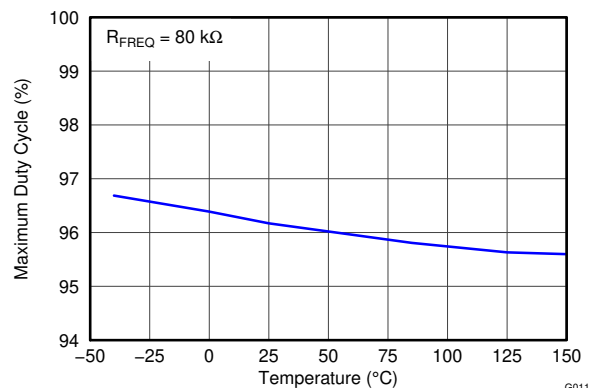
6-12. Maximum Duty Cycle vs Temperature
