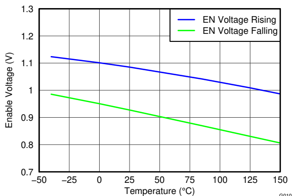
6-11. Enable Voltage vs Temperature
