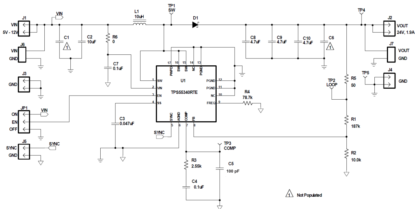
8-1. Boost Converter Application Schematic
