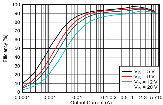
図 5-2. Efficiency vs Output Current, V_{OUT} = 5\text{ V} , PFM
