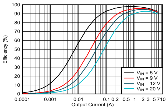
図 5-1. Efficiency vs Output Current, V_{OUT} = 5\text{ V} , FPWM
