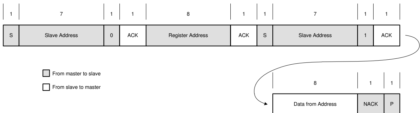
FIG 7-12. Single-byte Read
