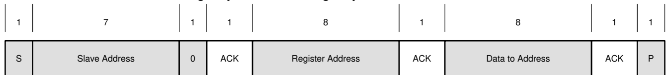
FIG 7-11. Single-byte Write
