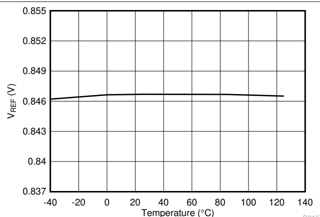
6-15. Reference Voltage vs Temperature ( V_{REF} = 0.846 V)
