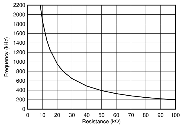
6-12. Switching Frequency vs Setting Resistance
