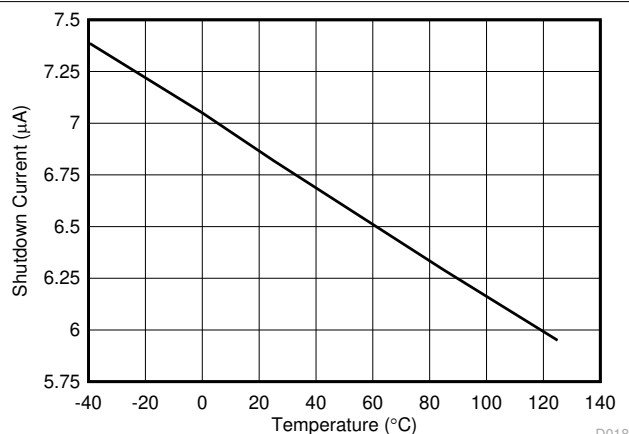
6-18. Shutdown Current vs Temperature
