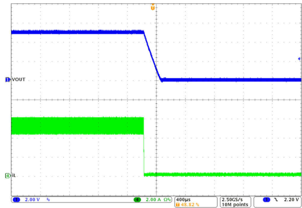
图 8-9. Shutdown Waveforms in V_{IN} = 12\text{ V} , V_{OUT} = 5\text{ V} , I_{OUT} = 5\text{ A} , FPWM
