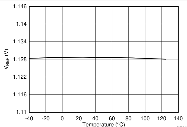
6-16. Reference Voltage vs Temperature ( V_{REF} = 1.129 V)
