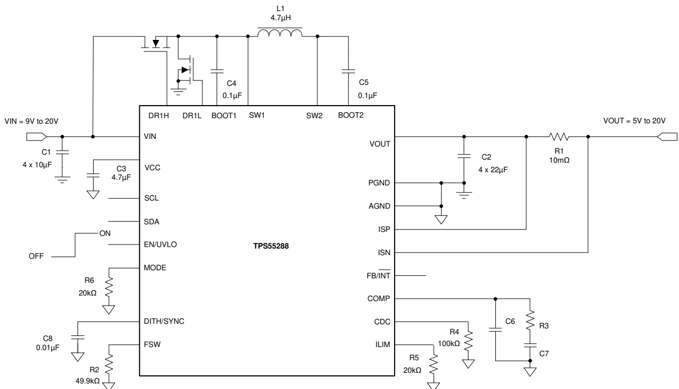
✎ 8-1. USB PD Power Supply With 9-V to 20-V Input Voltage
