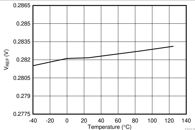
6-13. Reference Voltage vs Temperature ( V_{REF} = 0.282 V)
