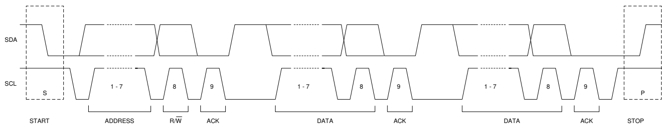
FIG 7-10. Slave Address and Data Direction
