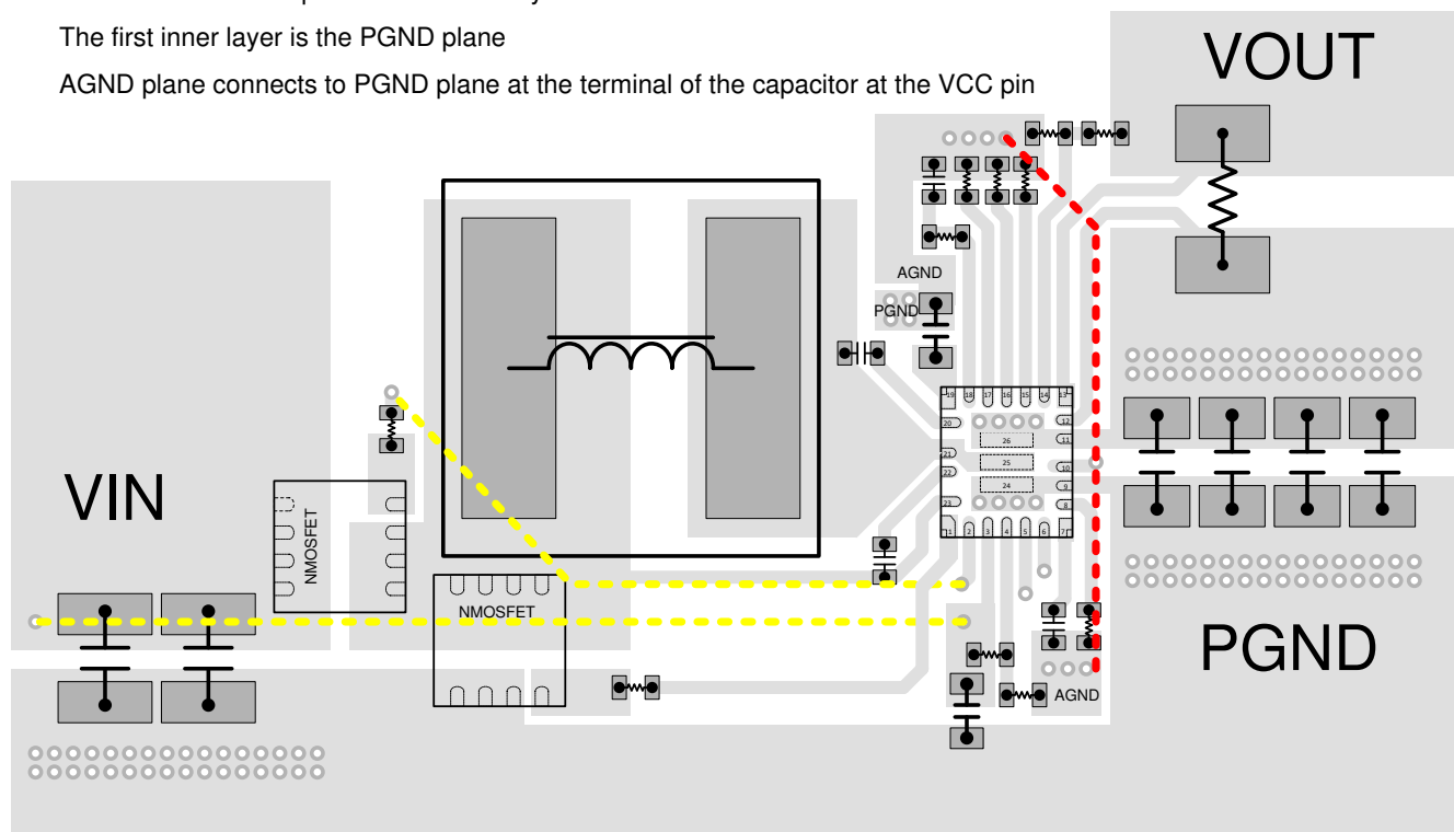
10-1. Layout Example
