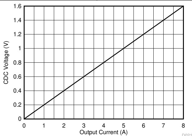
FIG 6-21. CDC Voltage vs Output Current with R SENSE = 10 mΩ
