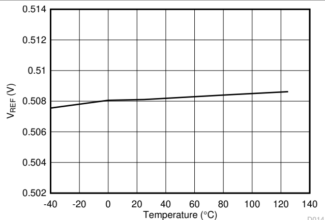
6-14. Reference Voltage vs Temperature ( V_{REF} = 0.508 V)
