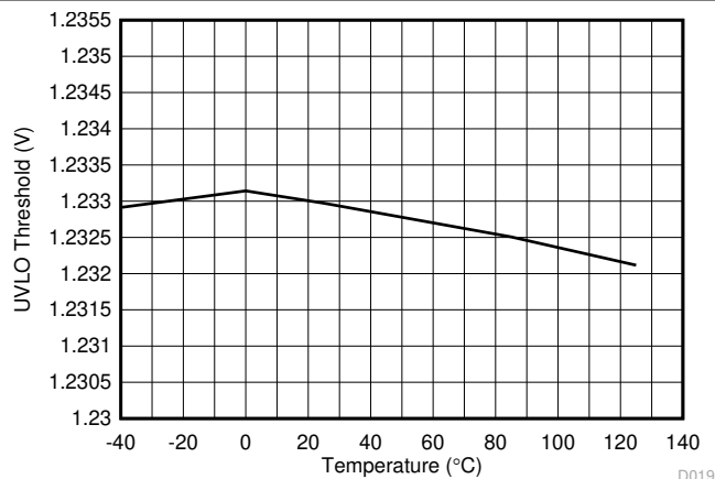
FIG 6-19. ENABLE/UVLO Rising Threshold vs Temperature
