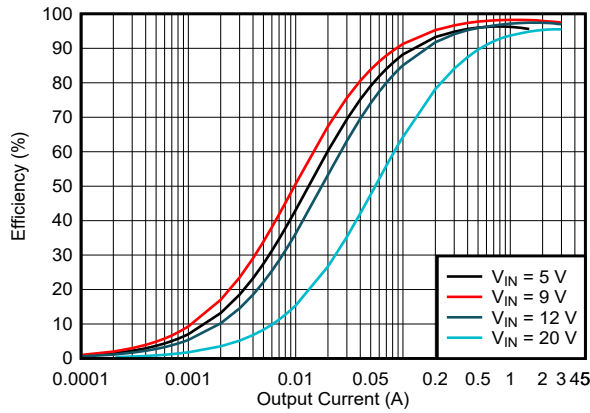
図 5-3. Efficiency vs Output Current, V_{OUT} = 9V , f_{SW} = 400\text{ kHz} , FPWM
