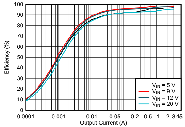
図 5-4. Efficiency vs Output Current, V_{OUT} = 9V , f_{SW} = 400\text{ kHz} , PFM
