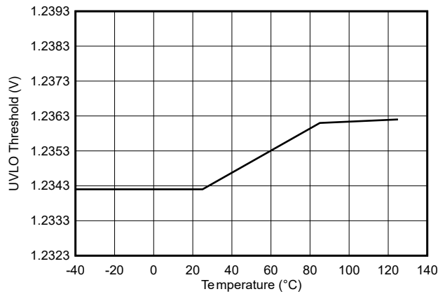
5-23. ENABLE/UVLO Rising Threshold vs Temperature
