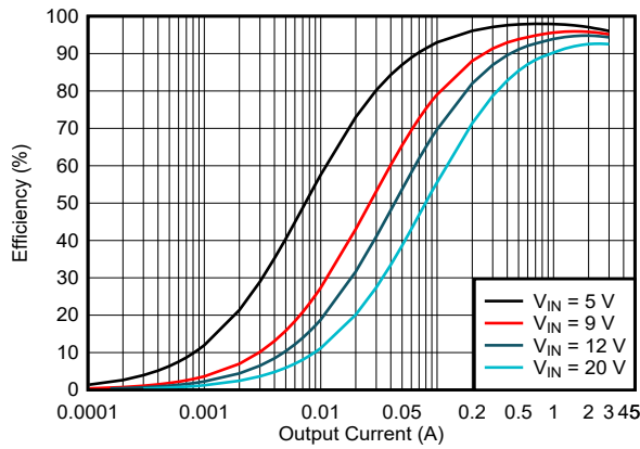
図 5-1. Efficiency vs Output Current, V_{OUT} = 5V , f_{SW} = 400\text{ kHz} , FPWM
