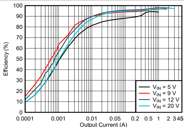
図 5-8. Efficiency vs Output Current, V_{OUT} = 15V , f_{SW} = 400\text{ kHz} , PFM
