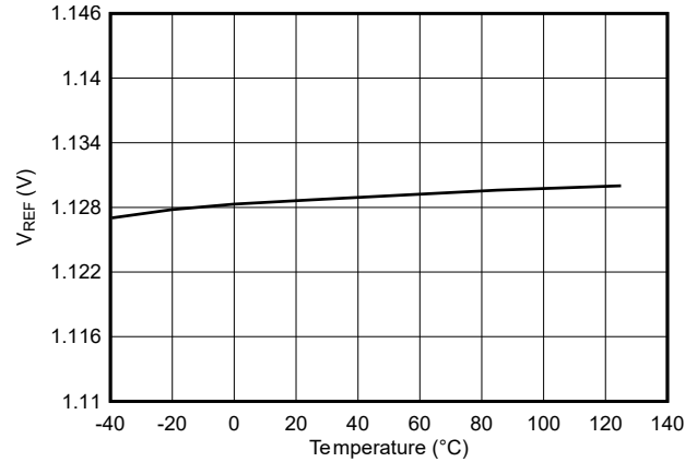
5-20. Reference Voltage vs Temperature ( V_{REF} = 1.129V )
