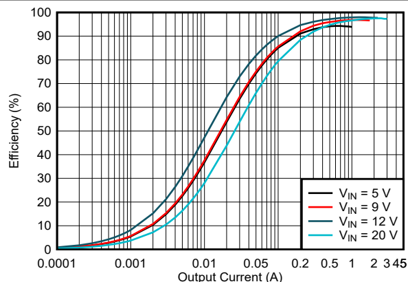
図 5-7. Efficiency vs Output Current, V_{OUT} = 15V , f_{SW} = 400\text{ kHz} , FPWM
