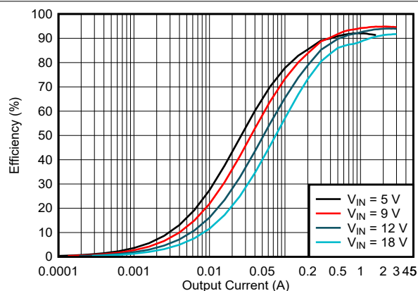
図 5-11. Efficiency vs Output Current, V_{OUT} = 9V , f_{SW} = 2\text{ MHz} , FPWM
