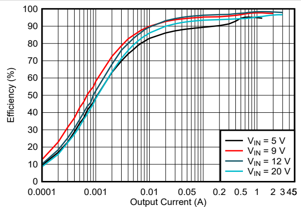
図 5-6. Efficiency vs Output Current, V_{OUT} = 12V , f_{SW} = 400\text{ kHz} , PFM
