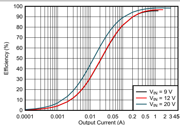
図 5-9. Efficiency vs Output Current, V_{OUT} = 20V , f_{SW} = 400\text{ kHz} , FPWM
