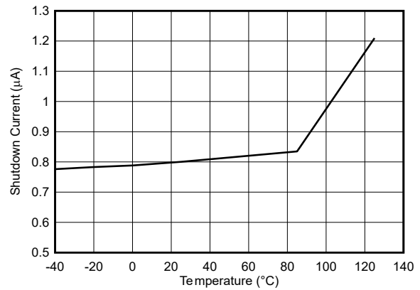
5-22. Shutdown Current vs Temperature
