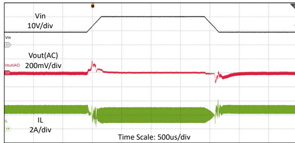
図 8-10. Line Transient Waveforms in V_{IN} = 9V to 20V , V_{OUT} = 12V , I_O = 2A with 200\mu s Slew Rate, FPWM
