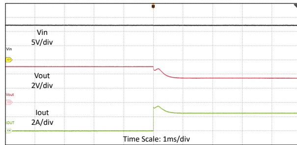
図 8-12. Output Current Limit Waveforms in V_{IN} = 12V , V_{OUT} = 5V , R_{LOAD} = 1.5\Omega , R_{SNS} = 20m\Omega FPWM
