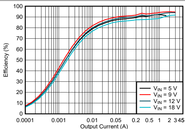
図 5-12. Efficiency vs Output Current, V_{OUT} = 9V , f_{SW} = 2\text{ MHz} , PFM
