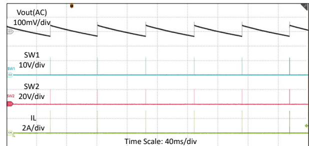
図 8-7. Switching Waveforms in V_{IN} = 12V , V_{OUT} = 20V , I_O = 0A , PFM
