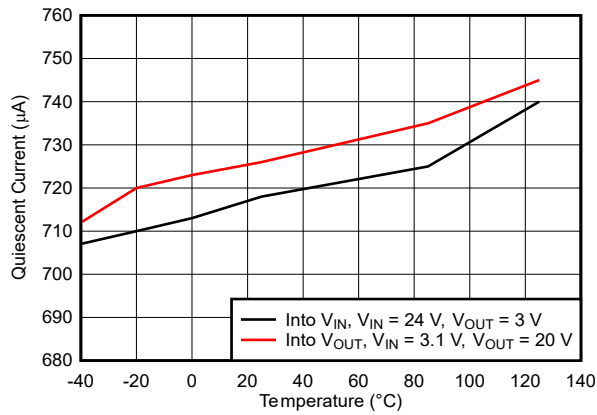
5-21. Quiescent Current vs Temperature
