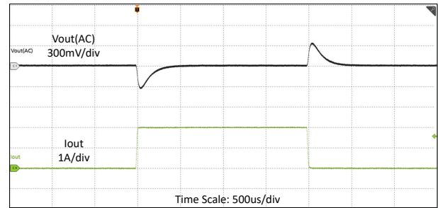
図 8-11. Load Transient Waveforms in V_{IN} = 12V , V_{OUT} = 5V , I_O = 0A to 2A with 20\mu s Slew Rate, FPWM
