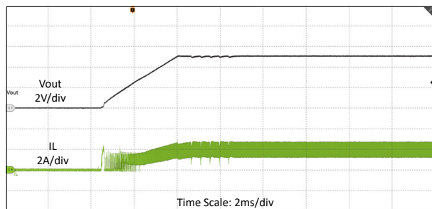
図 8-8. Start-up Waveforms in V_{IN} = 12V , V_{OUT} = 5V , R_{LOAD} = 2.5\Omega , FPWM
