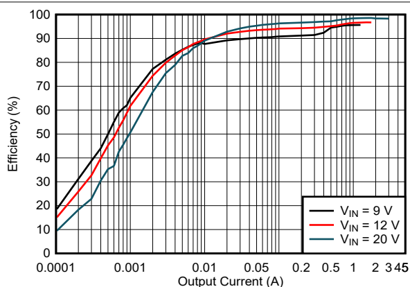
図 5-10. Efficiency vs Output Current, V_{OUT} = 20V , f_{SW} = 400\text{ kHz} , PFM
