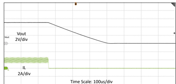
図 8-9. Shutdown Waveforms in V_{IN} = 12V , V_{OUT} = 5V , R_{LOAD} = 2.5\Omega , FPWM
