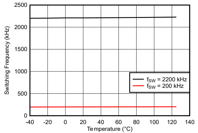
5-24. Switching Frequency vs Temperature
