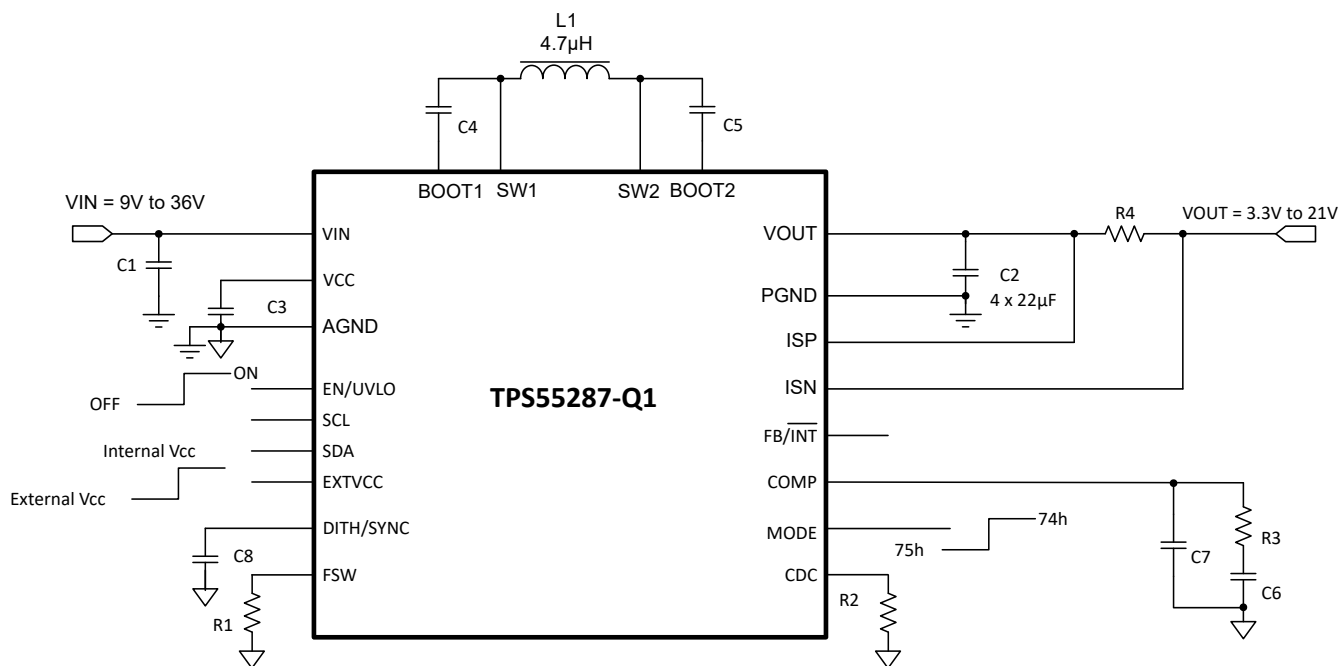
✎ 8-1. USB PD Power Supply With 9V to 36V Input Voltage
