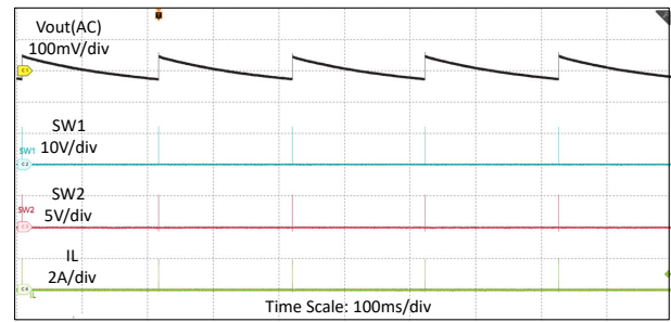
図 8-3. Switching Waveforms in V_{IN} = 12V , V_{OUT} = 5V , I_O = 0A , PFM
