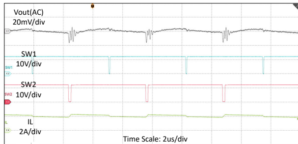
図 8-4. Switching Waveforms in V_{IN} = 12V , V_{OUT} = 12V , I_O = 2A , FPWM
