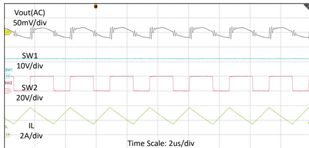
図 8-6. Switching Waveforms in V_{IN} = 12V , V_{OUT} = 20V , I_O = 1.5A , FPWM
