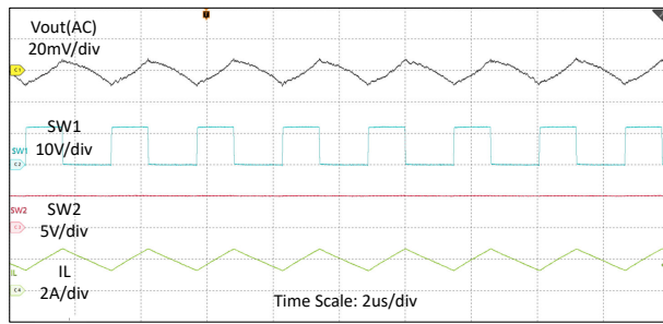
図 8-2. Switching Waveforms in V_{IN} = 12V , V_{OUT} = 5V , I_O = 2A , FPWM
