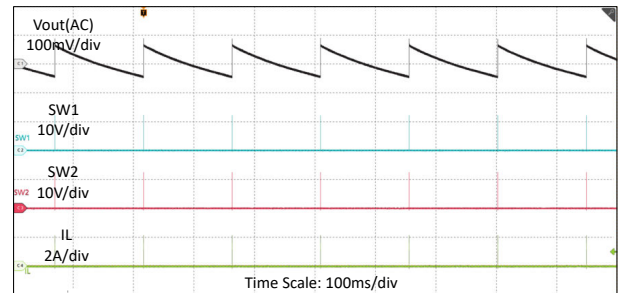
図 8-5. Switching Waveforms in V_{IN} = 12V , V_{OUT} = 12V , I_O = 0A , PFM
