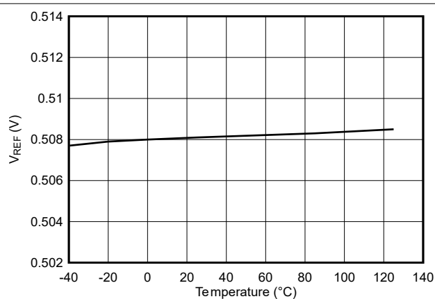
図 5-18. Reference Voltage vs Temperature ( V_{REF} = 0.508\text{ V} )
