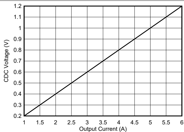
図 5-20. CDC Voltage vs Output Current with R SENSE = 10mΩ
