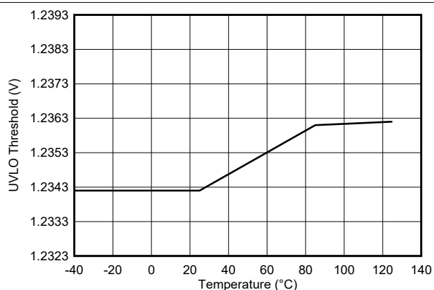
5-18. ENABLE/UVLO Rising Threshold vs Temperature
