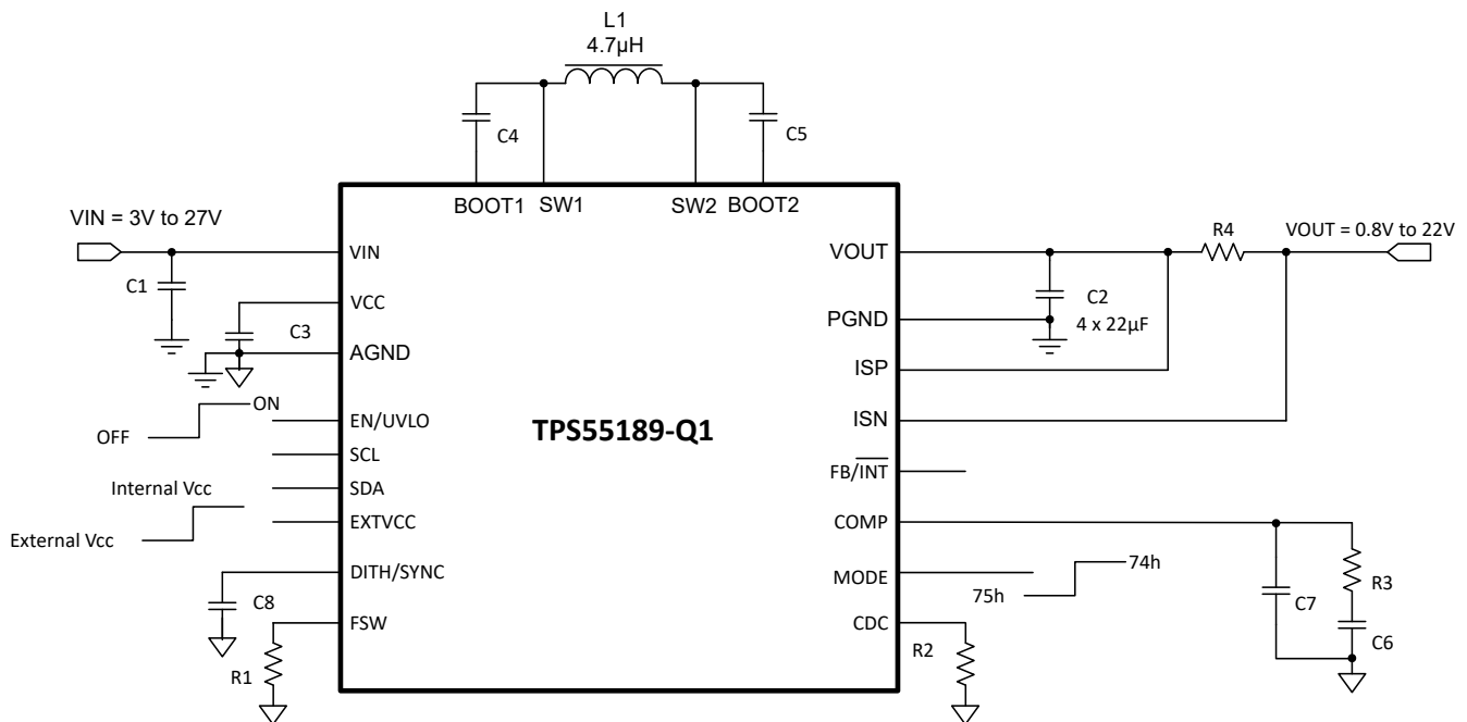
図 8-1. USB PD Power Supply With 9V to 27V Input Voltage
