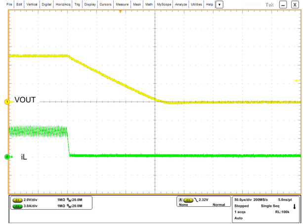
図 8-9. Shutdown Waveforms in V_{IN} = 12V , V_{OUT} = 5V , R_{LOAD} = 1.2\Omega , FPWM
