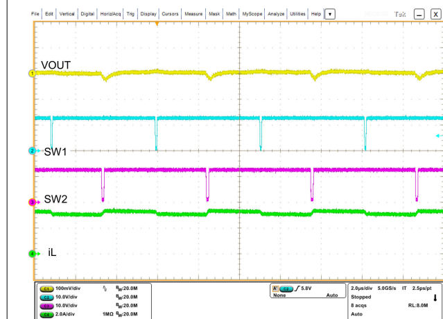
図 8-4. Switching Waveforms in V_{IN} = 12V , V_{OUT} = 12V , I_O = 3A , FPWM
