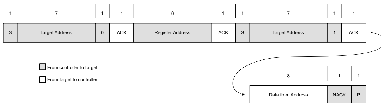
図 6-12. Single-byte Read
