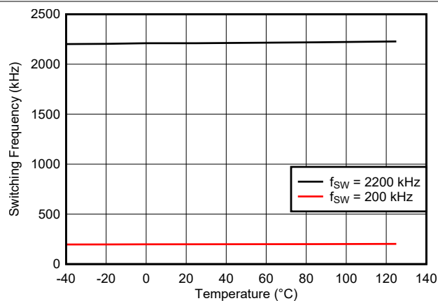
図 5-19. Switching Frequency vs Temperature
