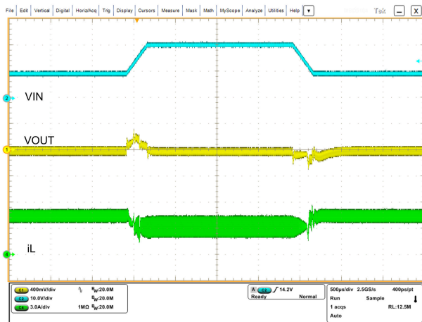
図 8-10. Line Transient Waveforms in V_{IN} = 9V to 20V , V_{OUT} = 12V , I_O = 3A with 200\mu s Slew Rate, FPWM
