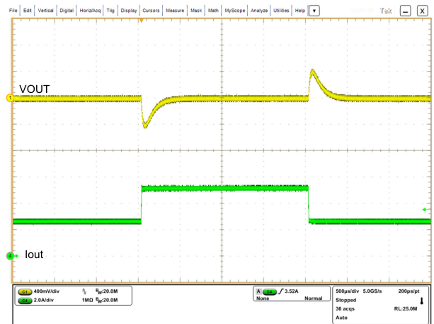
図 8-11. Load Transient Waveforms in V_{IN} = 12V , V_{OUT} = 5V , I_O = 2.5A to 5A with 20\mu s Slew Rate, FPWM
