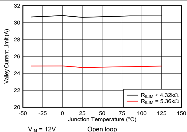
图 5-20. Valley Current Limit versus Junction Temperature (Low R_{ILIM} )
