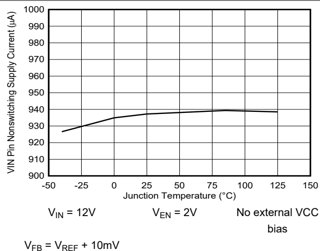
图 5-19. VIN Pin Nonswitching Quiescent Current versus Junction Temperature
