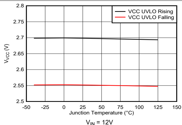
图 5-24. VCC Pin Undervoltage Lockout versus Junction Temperature
