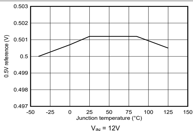
図 5-16. 0.5V Reference Voltage versus Junction Temperature
