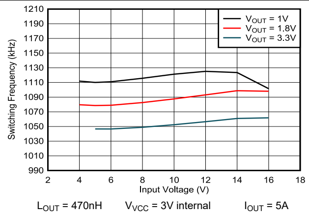
図 5-10. 1100kHz Switching Frequency versus Input Voltage
