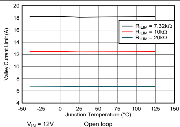
图 5-21. Valley Current Limit versus Junction Temperature (High R_{ILIM} )
