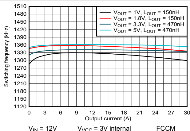
図 5-15. 1400kHz Switching Frequency versus Output Current
