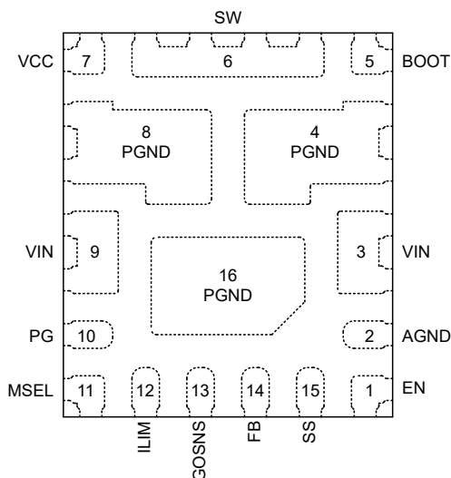
図 4-1. RZR Package 16-Pin WQFN-FCRLF Top View
