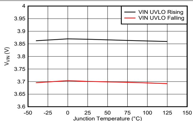
图 5-23. VIN Pin Undervoltage Lockout versus Junction Temperature
