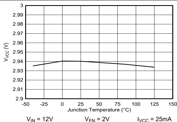
図 5-17. VCC Pin Output Voltage versus Junction Temperature
