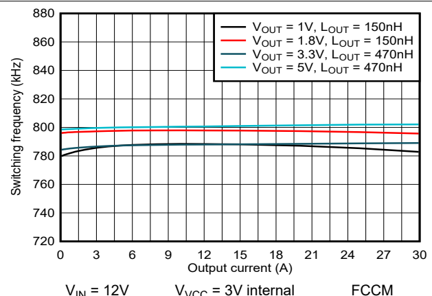
図 5-12. 800kHz FCM Switching Frequency versus Output Current
