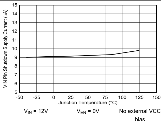
図 5-18. VIN Pin Shutdown Quiescent Current versus Junction Temperature
