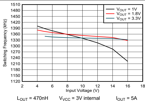
図 5-11. 1400kHz Switching Frequency versus Input Voltage
