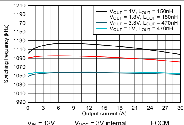
図 5-14. 1100kHz Switching Frequency versus Output Current
