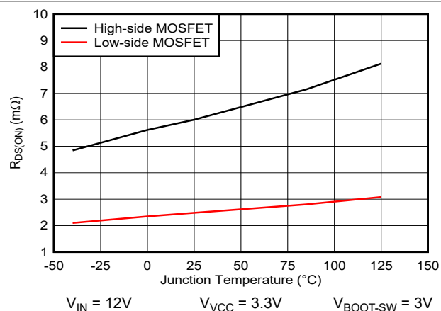
图 5-22. MOSFET R_{DS(ON)} versus Junction Temperature
