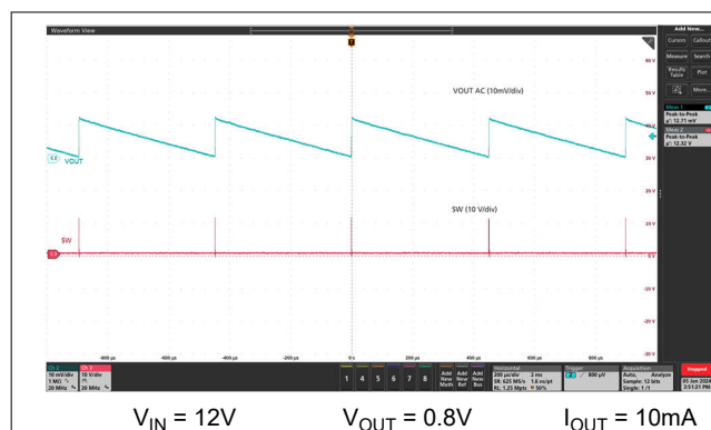
図 7-8. Output Voltage Ripple – Skip-mode
