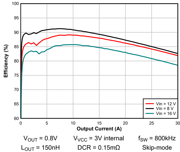
図 7-2. Efficiency – Skip-mode
