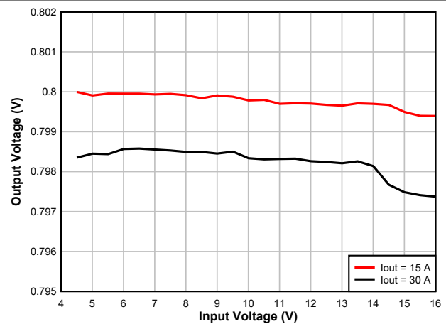
図 7-5. Line Regulation
