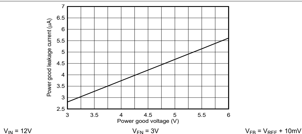
図 5-31. Power-Good Leakage Current versus Power-Good Voltage
