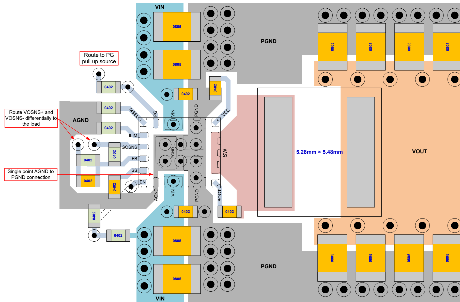
図 7-12. Layout Recommendation
