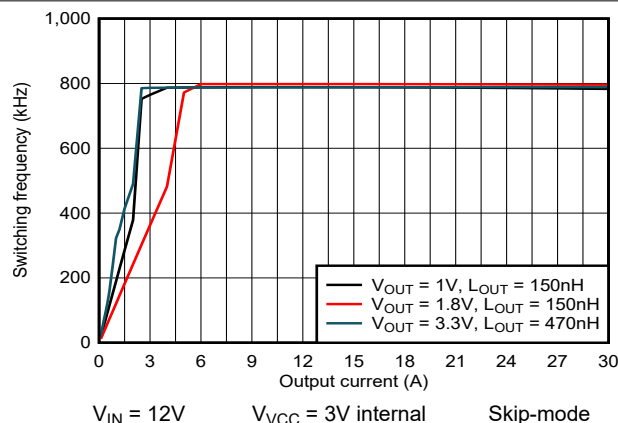
図 5-13. 800kHz Skip-mode Switching Frequency versus Output Current
