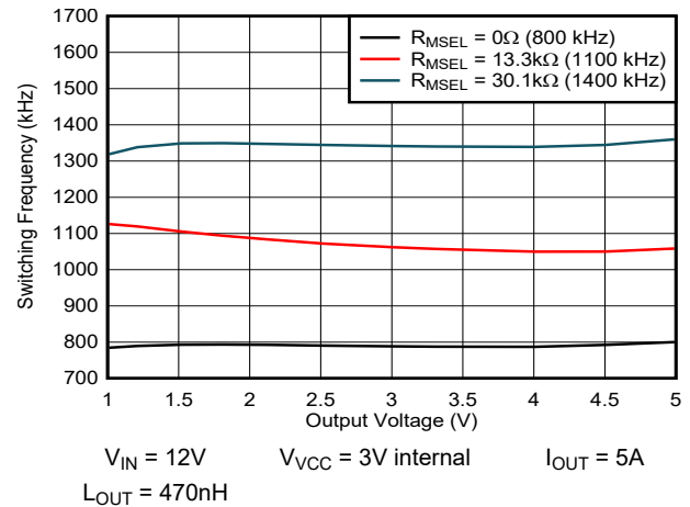
図 5-8. Switching Frequency versus Output Voltage
