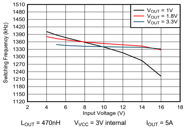
5-15. 1400kHz Switching Frequency versus Input Voltage
