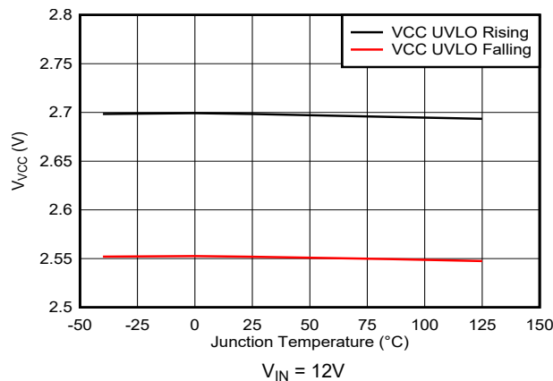
5-29. VCC Pin Undervoltage Lockout versus Junction Temperature
