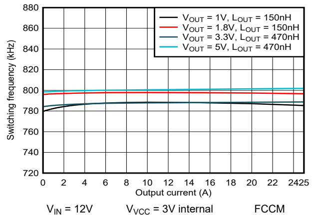
5-16. 800kHz FCCM Switching Frequency versus Output Current
