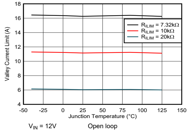
5-26. Valley Current Limit versus Junction Temperature (High R_{ILIM} )
