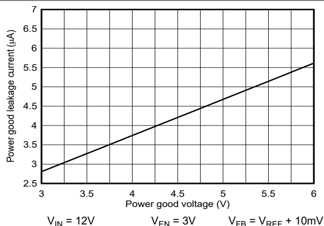
図 5-38. Power-Good Leakage Current versus Power-Good Voltage
