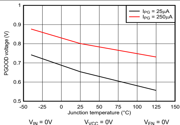
図 5-37. Power-Good Clamp Voltage versus Junction Temperature
