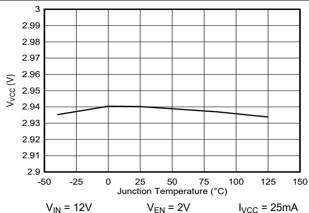
FIG 5-22. VCC Pin Output Voltage versus Junction Temperature
