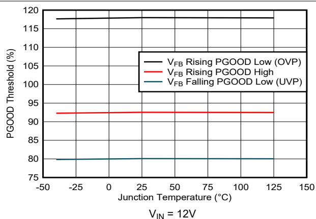
5-36. Power-Good Thresholds versus Junction Temperature ( V_{REF} = 0.9V )
