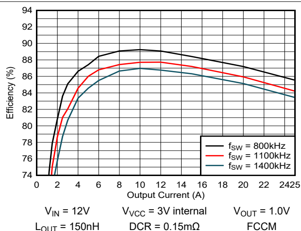
図 5-4. Efficiency versus f_{SW} With V_{OUT} = 1.0V
