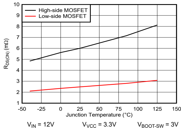
5-27. MOSFET R_{DS(ON)} versus Junction Temperature
