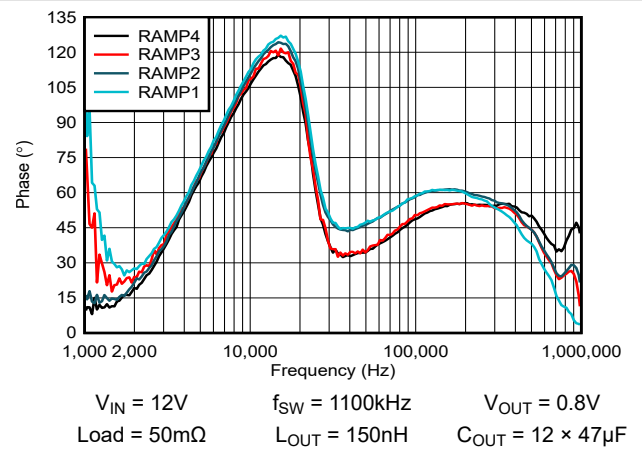
6-6. Phase versus Ramp Setting - VREF = 0.5V
