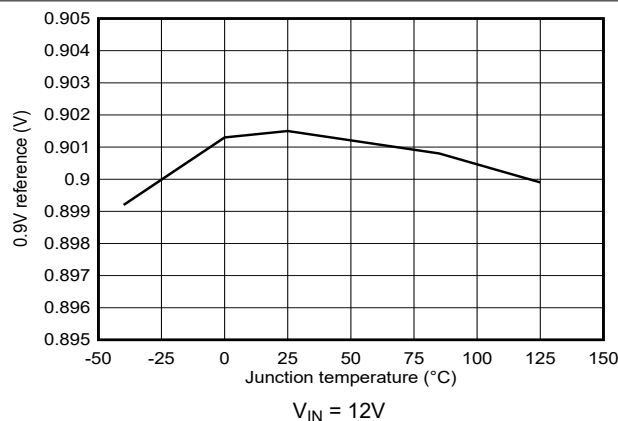
FIG 5-21. 0.9V Reference Voltage versus Junction Temperature
