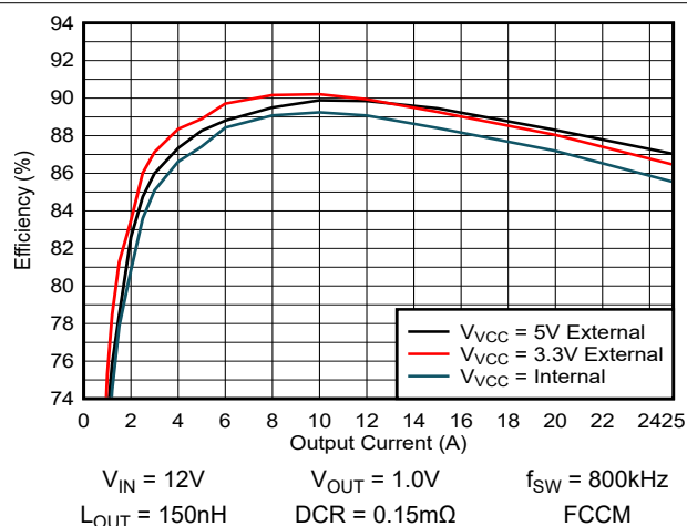
図 5-6. Efficiency versus VCC Bias With V_{OUT} = 1.0V
