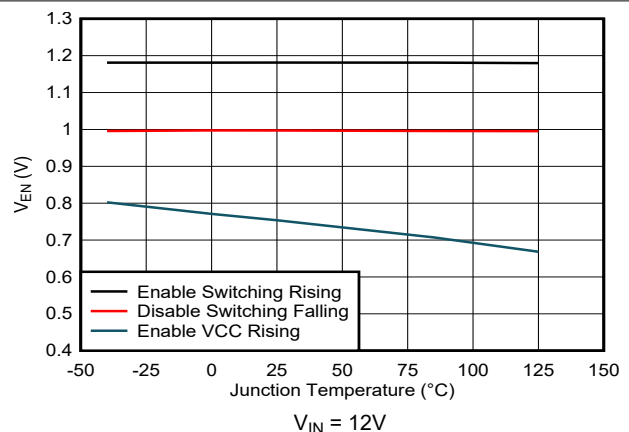
5-30. EN Pin Thresholds versus Junction Temperature
