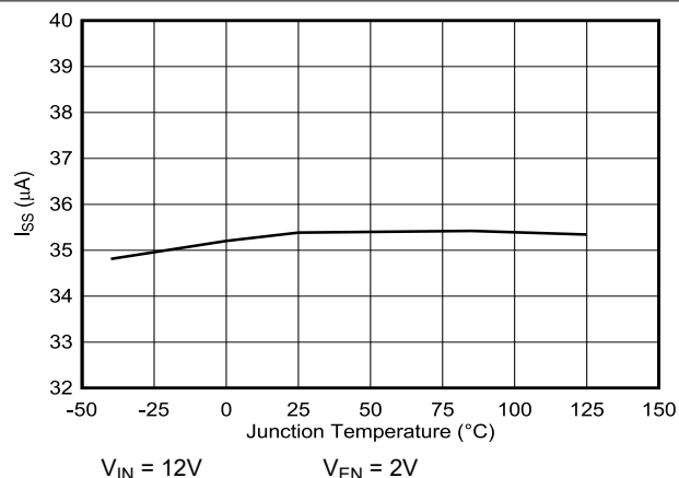
5-32. SS Pin Output Current versus Junction Temperature
