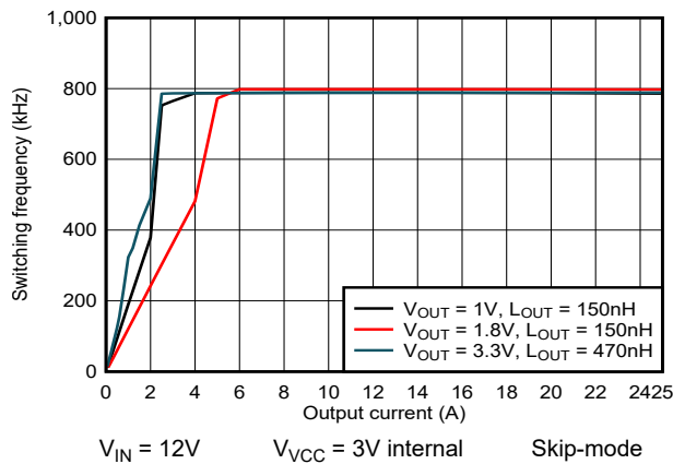
5-17. 800kHz Skip-mode Switching Frequency versus Output Current
