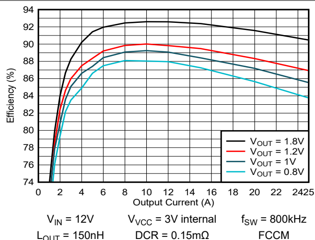
図 5-2. Efficiency With V_{OUT} \leq 1.8V
