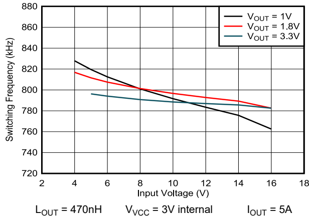
5-13. 800kHz Switching Frequency versus Input Voltage
