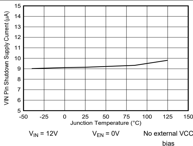
FIG 5-23. VIN Pin Shutdown Quiescent Current versus Junction Temperature
