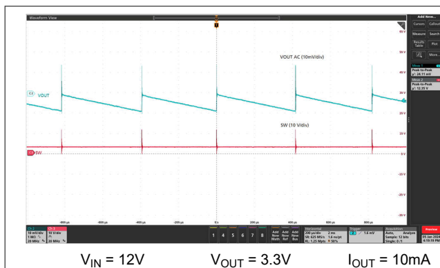
図 7-8. Output Voltage Ripple – Skip-mode
