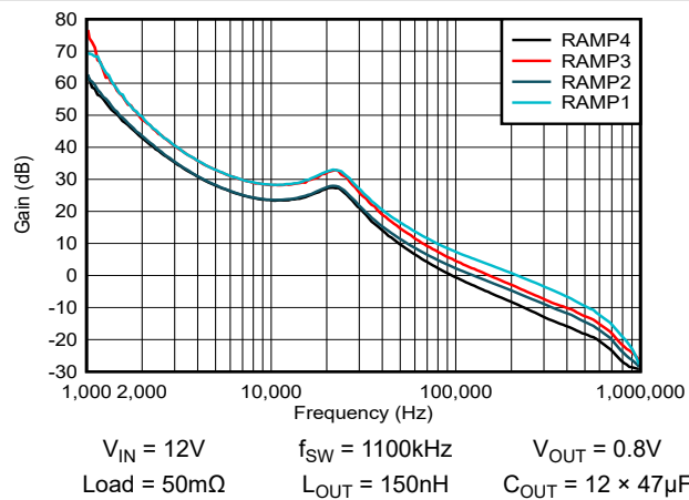
6-5. Gain versus Ramp Setting - VREF = 0.5V
