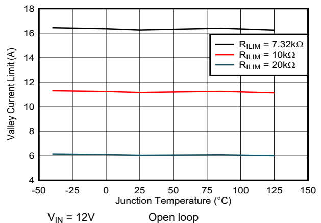
5-26. Valley Current Limit versus Junction Temperature (High R_{ILIM} )
