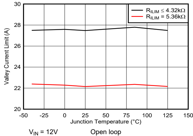
5-25. Valley Current Limit versus Junction Temperature (Low R_{ILIM} )
