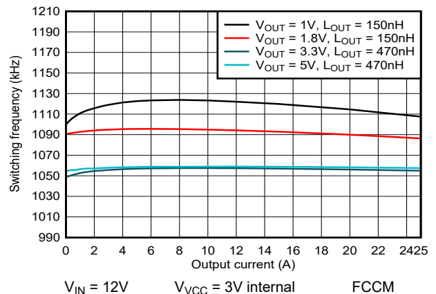
5-18. 1100kHz Switching Frequency versus Output Current
