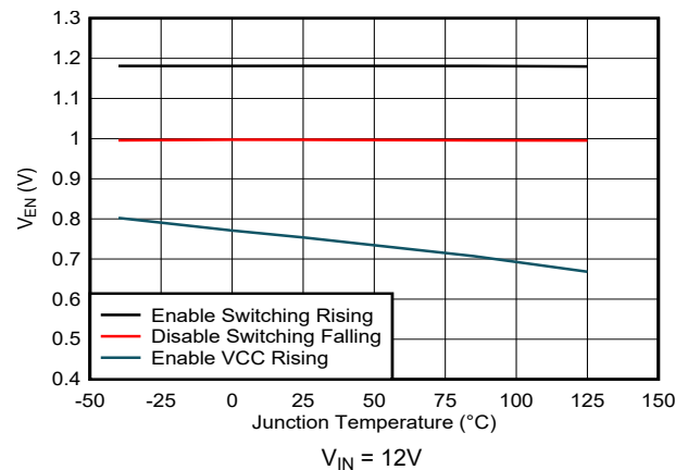
5-30. EN Pin Thresholds versus Junction Temperature
