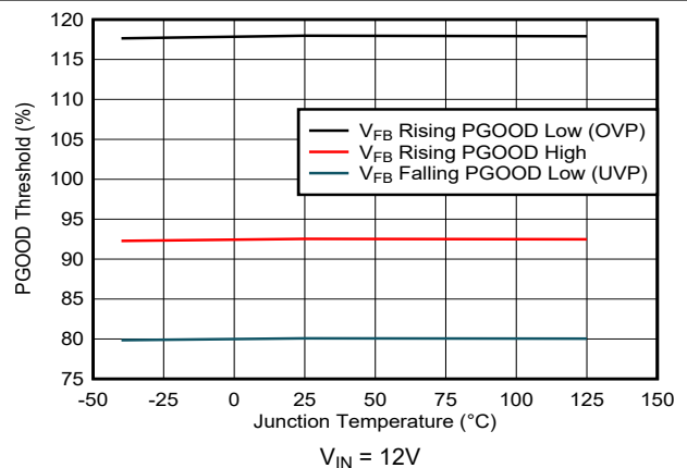
5-36. Power-Good Thresholds versus Junction Temperature ( V_{REF} = 0.9V )
