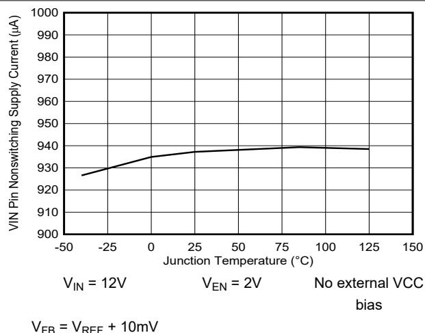
FIG 5-24. VIN Pin Nonswitching Quiescent Current versus Junction Temperature
