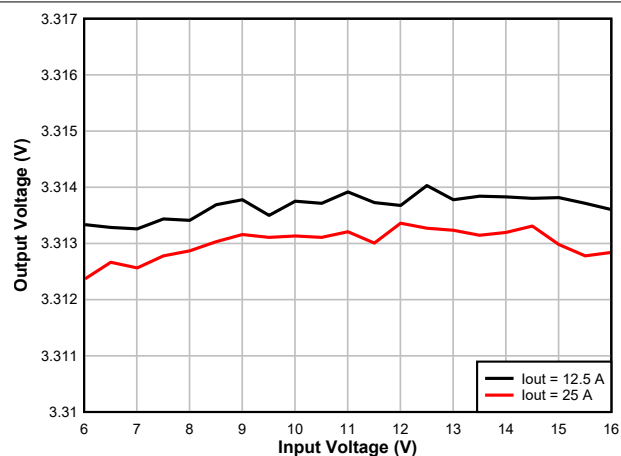
図 7-5. Line Regulation
