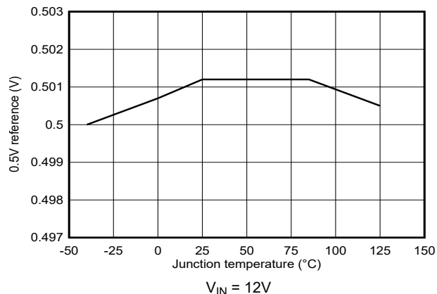
FIG 5-20. 0.5V Reference Voltage versus Junction Temperature
