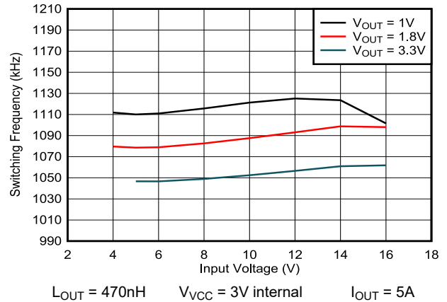
5-14. 1100kHz Switching Frequency versus Input Voltage
