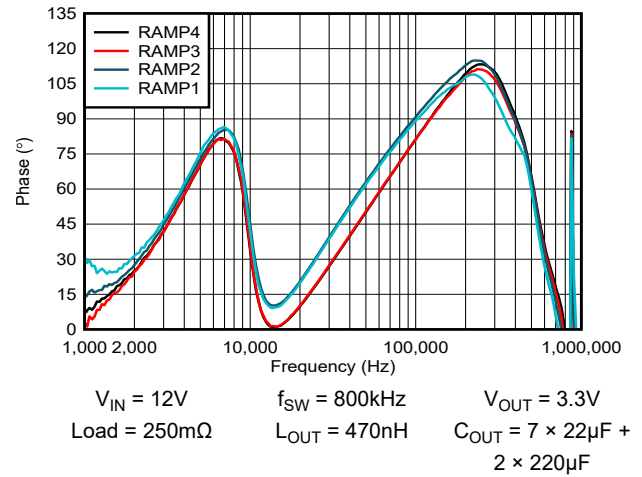
6-4. Phase versus Ramp Setting - VREF = 0.9V
