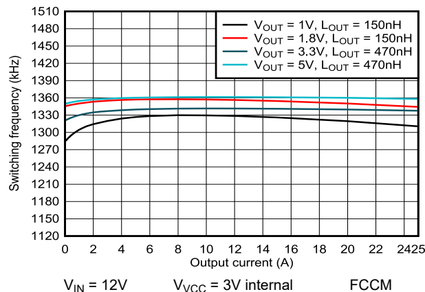
FIG 5-19. 1400kHz Switching Frequency versus Output Current
