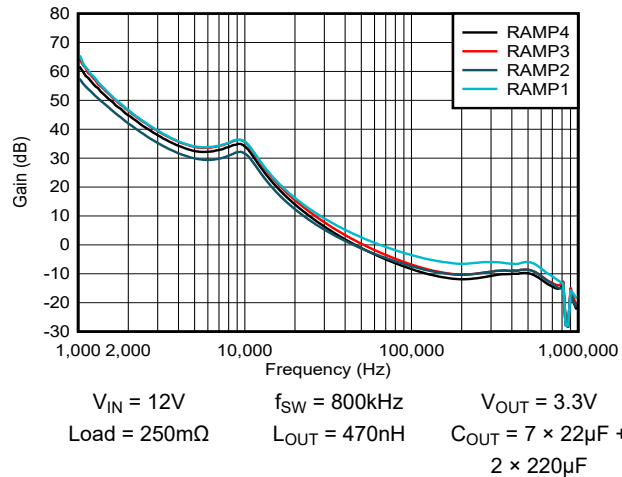
6-3. Gain versus Ramp Setting - VREF = 0.9V
