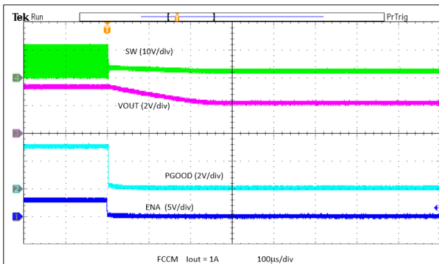
Figure 8-20. Prebias Power-Down
