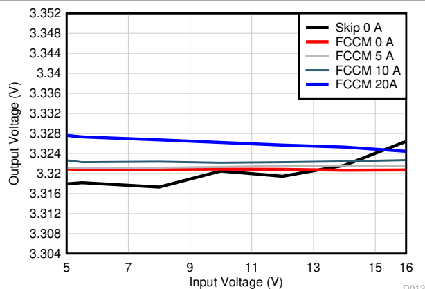
8-12. Output Voltage vs Input Voltage VCC = Int
