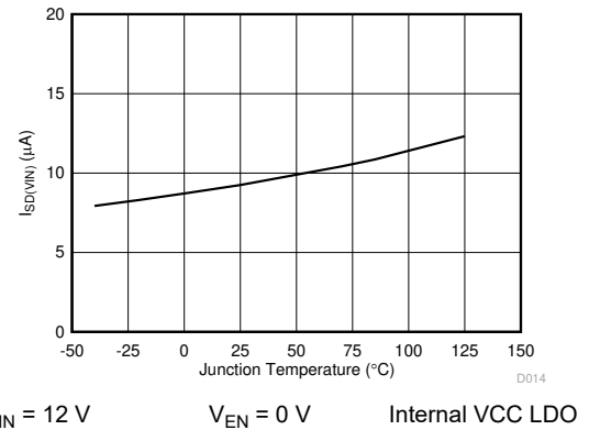
Figure 6-8. I_{SD(VIN)} vs Junction Temperature
