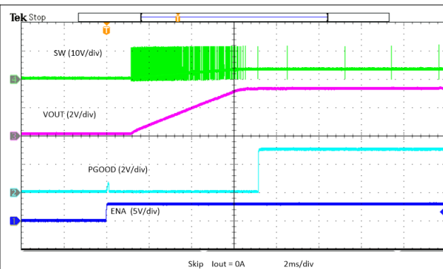
Figure 8-21. Enable Power Up, Skip
