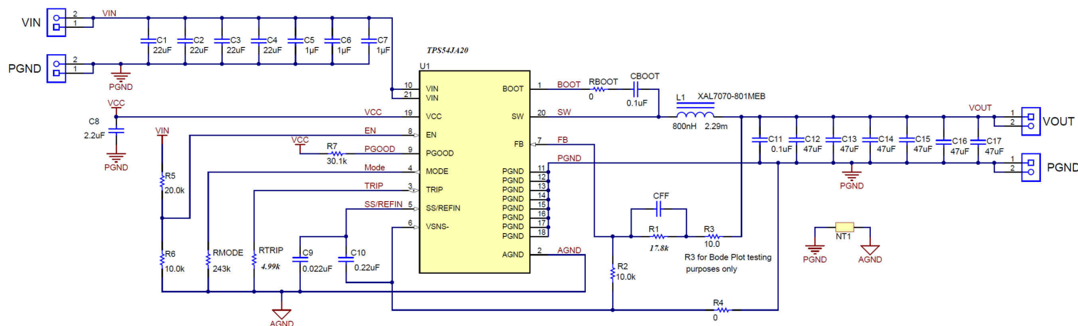
8-1. Application Circuit Diagram
