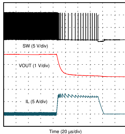
図 7-30. Short Circuit Response
