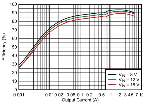
Figure 7-4. Efficiency – 1100 kHz, FFCM, External 3.3-V VCC, 4.7- \Omega R_{BOOT}
