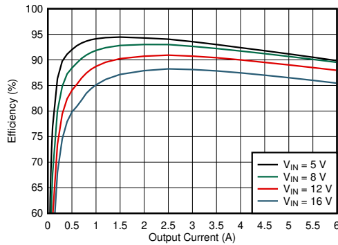
Figure 7-2. Efficiency – 1100 kHz, FFCM
