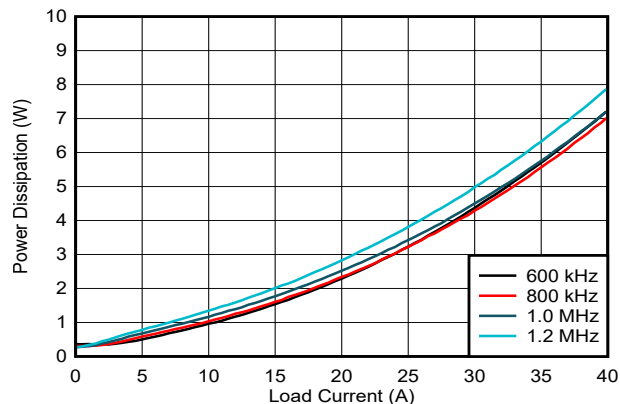
図 7-3. Power Dissipation vs Output Current
