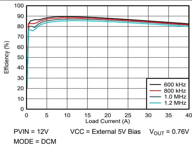
図 5-5. Efficiency vs Output Current
