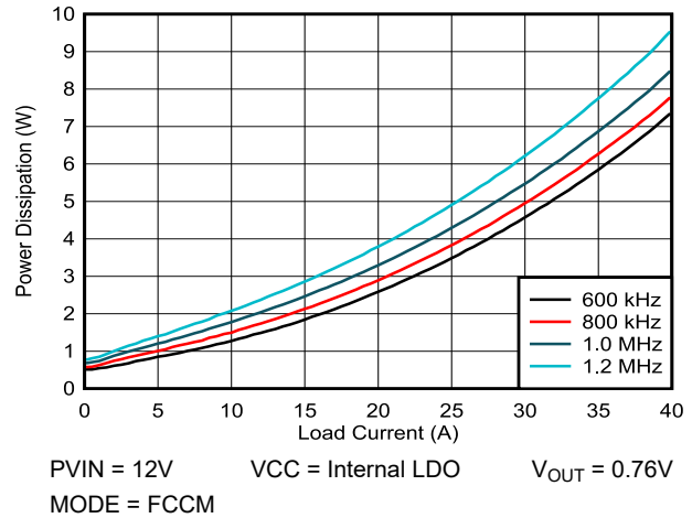
図 5-2. Power Dissipation vs Output Current
