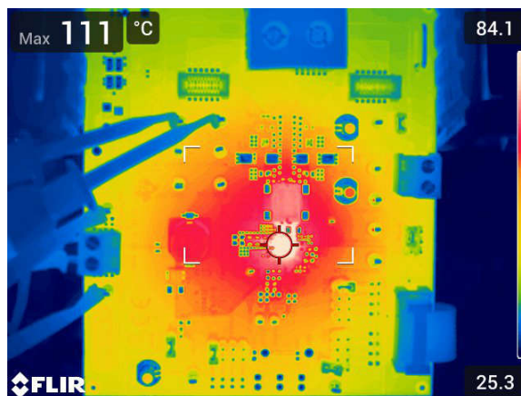
図 7-18. Thermal Characteristics, 600kHz FCCM, Internal LDO, 40A Load
