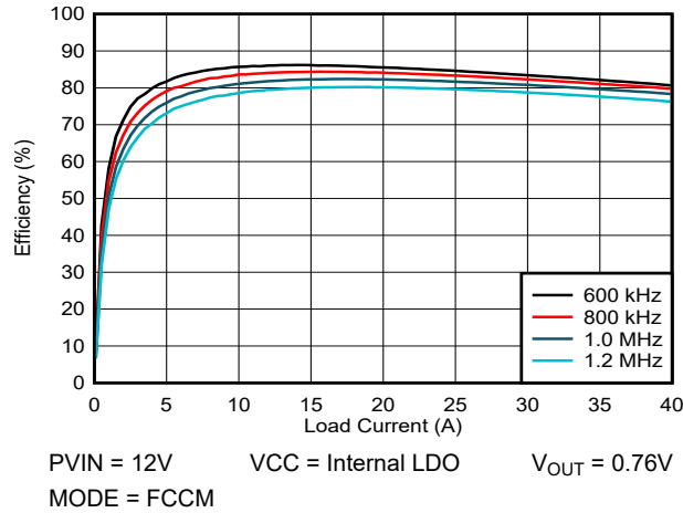
図 5-1. Efficiency vs Output Current
