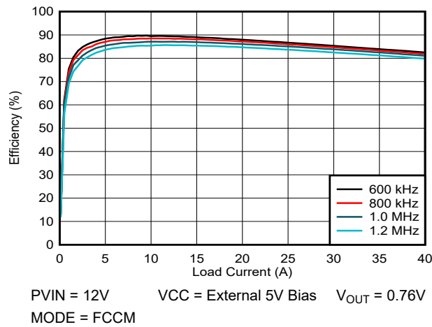
図 5-3. Efficiency vs Output Current
