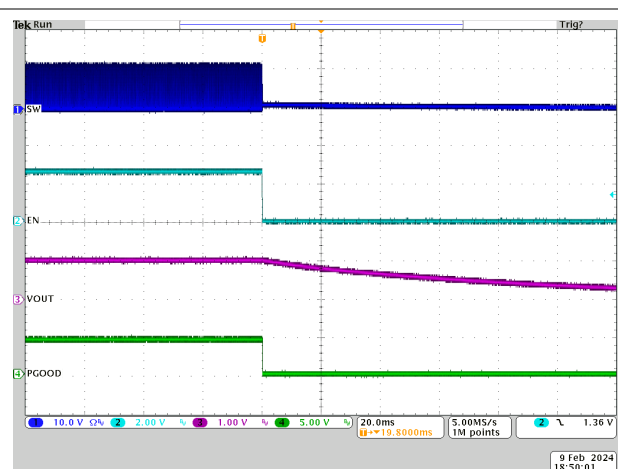
図 7-13. ENABLE Shutdown Waveform, PVIN = 12V, VOUT = 1.1V
