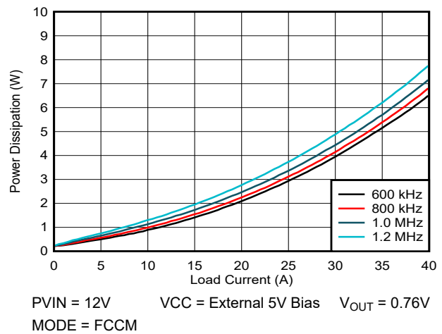
図 5-4. Power Dissipation vs Output Current
