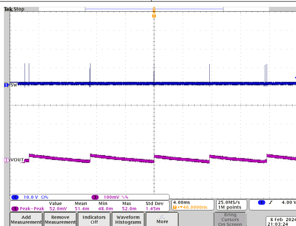
図 7-16. Output Voltage Ripple, DCM, No load, PVIN = 12V, VOUT = 1.1V
