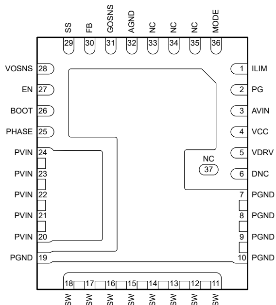
図 4-2. RXX 37-Pin WQFN-FCRLF Package (Bottom View)
