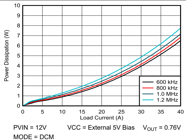
図 5-6. Power Dissipation vs Output Current
