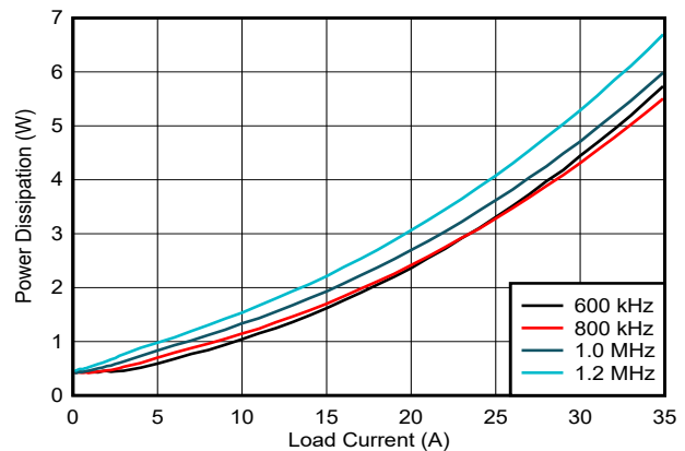
8-3. Power Dissipation, FFCM, Internal LDO
