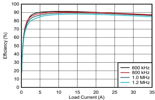
8-4. Efficiency, FFCM, External 5-V Bias
