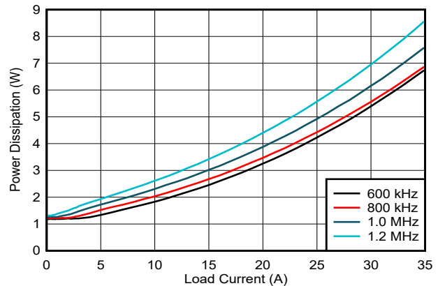
8-3. Power Dissipation, FFCM, Internal LDO
