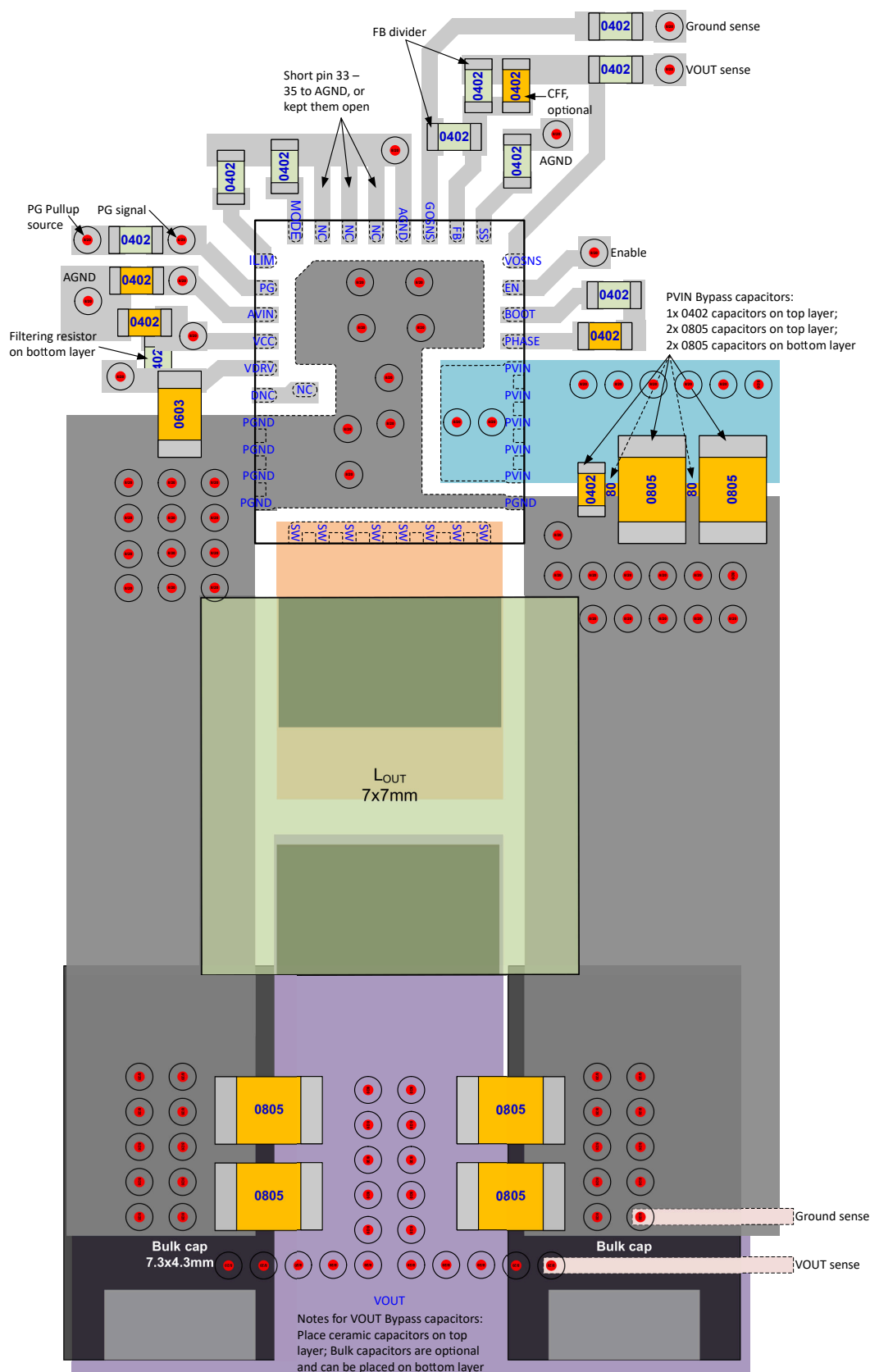
☒ 8-17. Layout Recommendation
