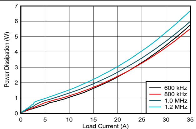
8-5. Power Dissipation, FFCM, External 5-V Bias
