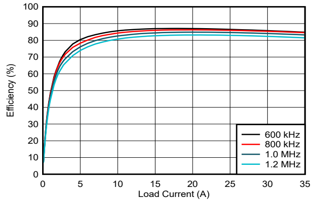
8-2. Efficiency, FFCM, Internal LDO
