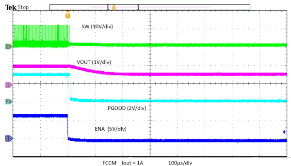
8-15. Prebias Power-Down
