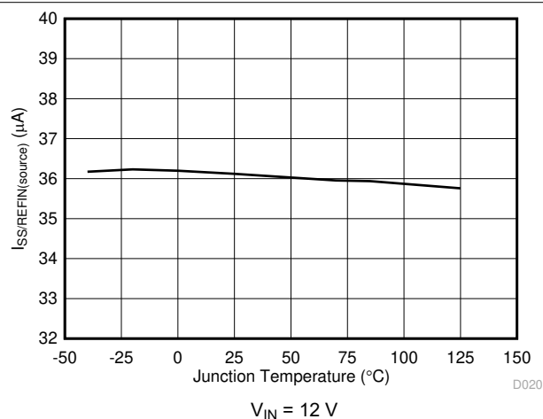
6-12. I_{SS(source)} vs Junction Temperature
