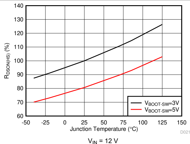
FIG 6-13. R_{DS(on)(HS)} vs Junction Temperature
