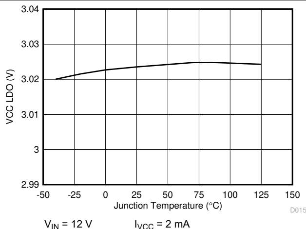
6-9. VCC LDO vs Junction Temperature
