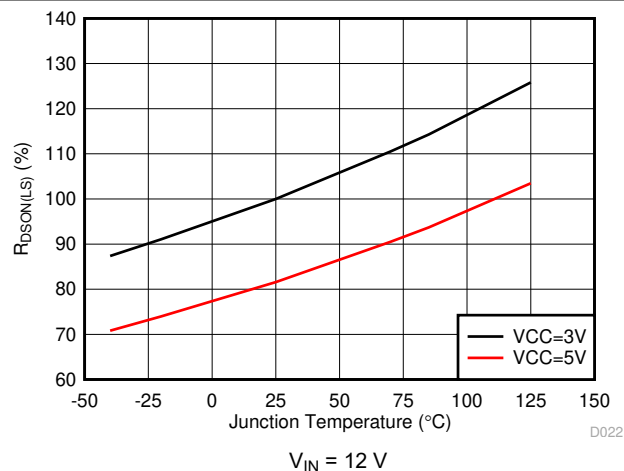
FIG 6-14. R_{DS(on)(LS)} vs Junction Temperature
