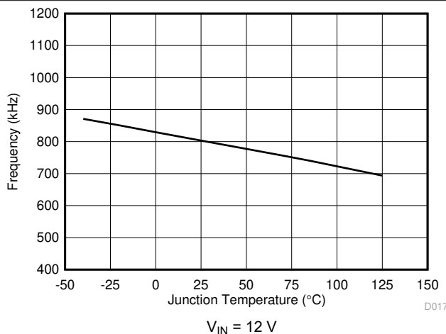
6-11. Switching Frequency vs Junction Temperature
