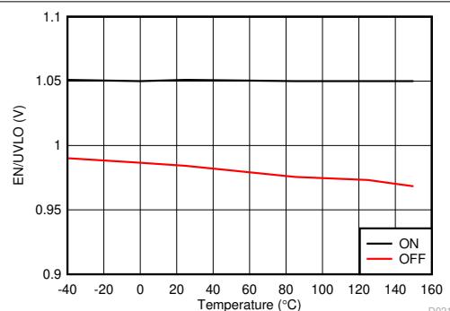
FIG 6-22. EN/UVLO Thresholds vs Junction Temperature
