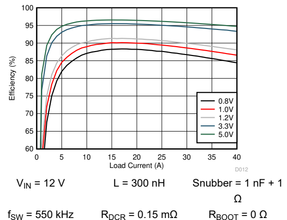
FIG 6-12. TPS546D24S Efficiency vs. Output Current
