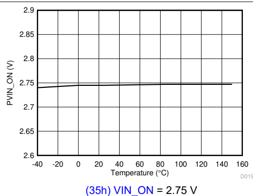
FIG 6-20. Turnon Voltage vs Junction Temperature
