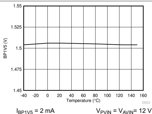
FIG 6-19. BP1V5 Voltage vs Junction Temperature
