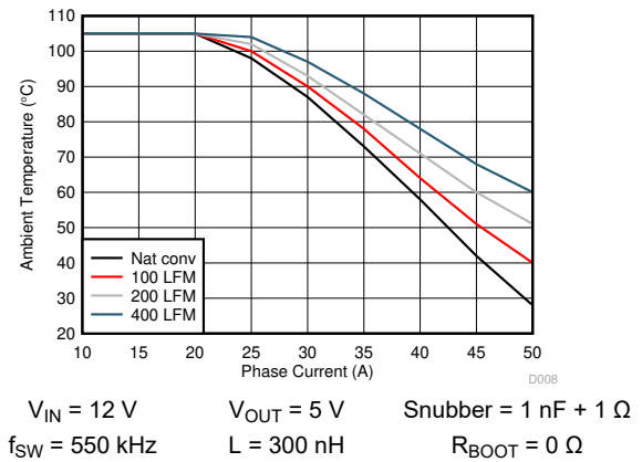
FIG 6-8. TPS546D24S Safe Operating Area
