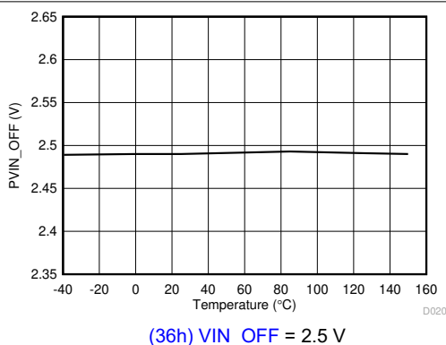
FIG 6-21. Turnoff Voltage vs Junction Temperature
