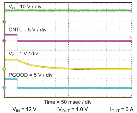
8-7. Shutdown from CNTL
