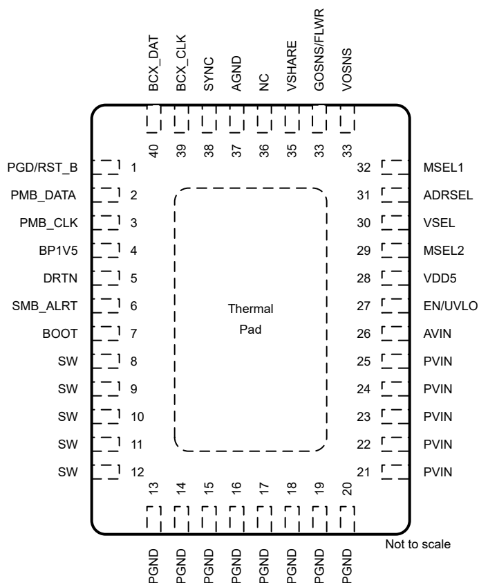
図 5-1. 40-Pin LQFN-CLIP with Exposed Thermal Pad RVF Package (Top View)
