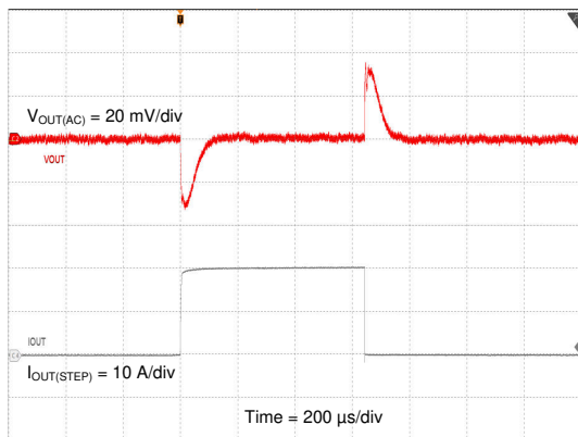
Figure 8-14. Load Regulation
