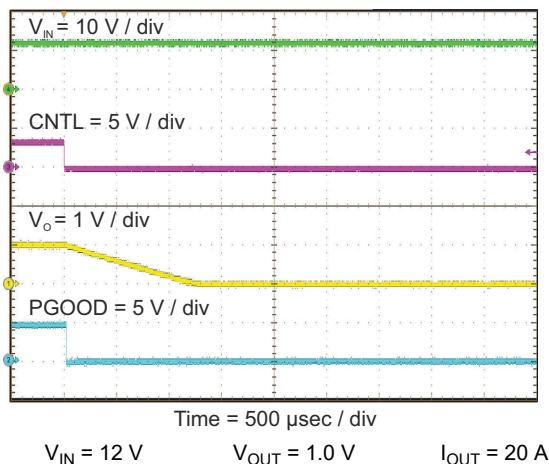
8-6. Shutdown from CNTL
