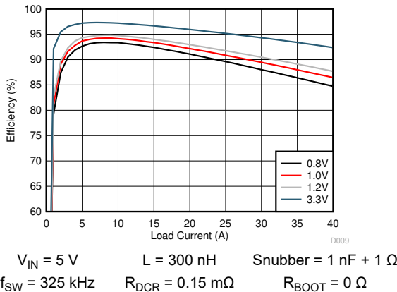
FIG 6-9. TPS546D24S Efficiency vs. Output Current
