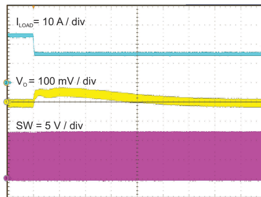
8-9. Load Transient Response
