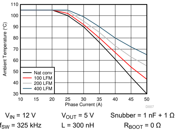
FIG 6-7. TPS546D24S Safe Operating Area
