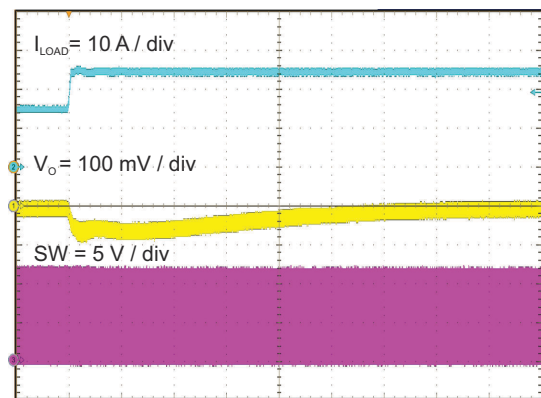
8-8. Load Transient Response
