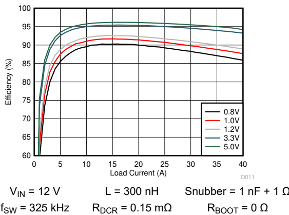
FIG 6-11. TPS546D24S Efficiency vs. Output Current
