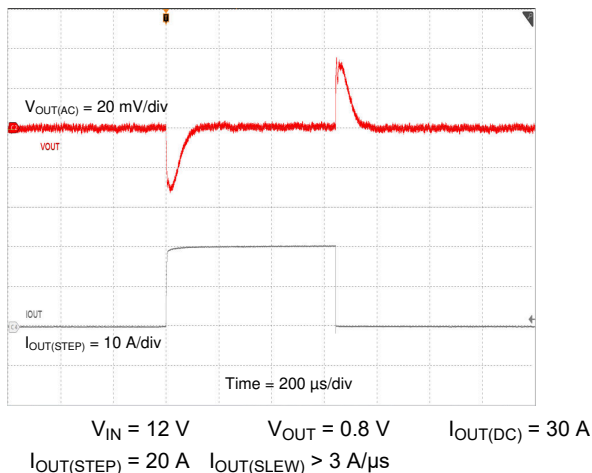
Figure 8-16. Load Transient Response
