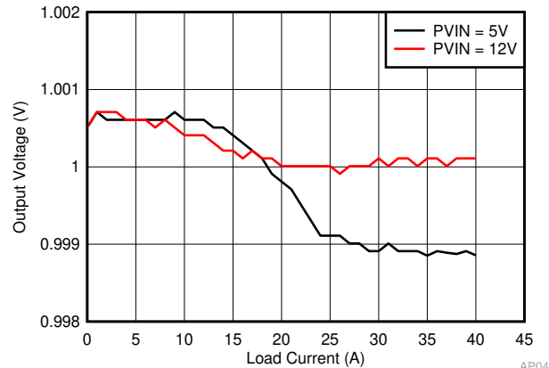
8-3. Load Regulation
