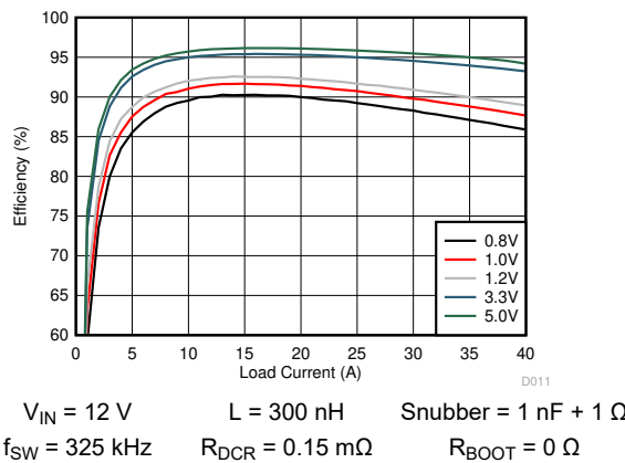
Figure 6-11. TPS546D24S Efficiency vs. Output Current
