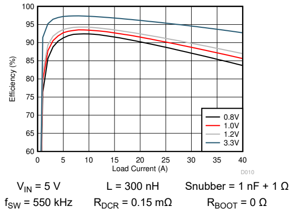
FIG 6-10. TPS546D24S Efficiency vs. Output Current
