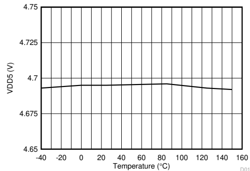
Figure 6-18. VDD5 Voltage vs Junction Temperature I_{VDD5} = 10\text{ mA} V_{PVIN} = V_{AVIN} = 12\text{ V}
