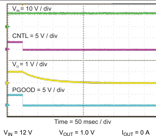
8-7. Shutdown from CNTL
