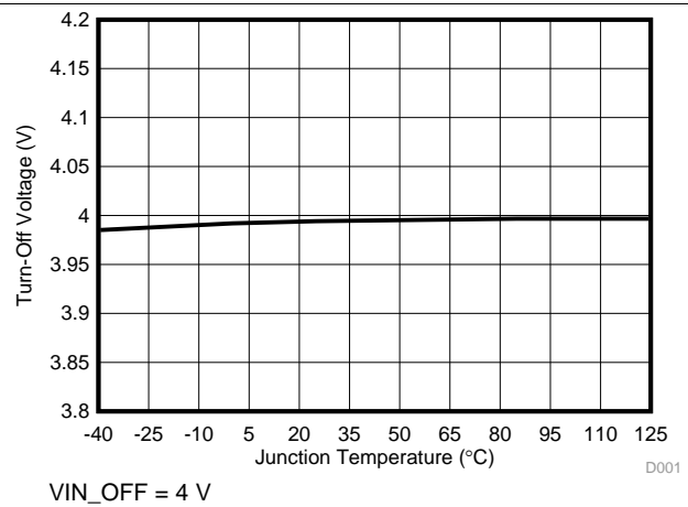
FIG 14. Turnoff Voltage vs Junction Temperature
