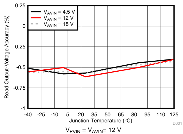
FIG 16. READ_VOUT Accuracy vs Junction Temperature
