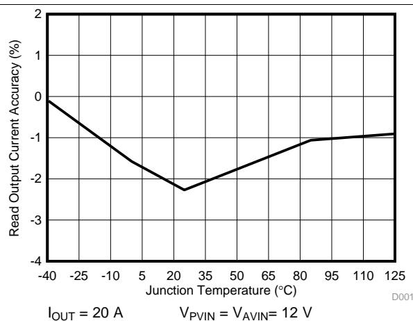
FIG 15. READ_IOUT Accuracy vs Junction Temperature
