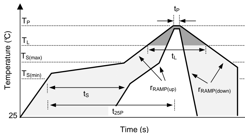
FIG 53. Recommended Reflow-Oven Thermal Profile
