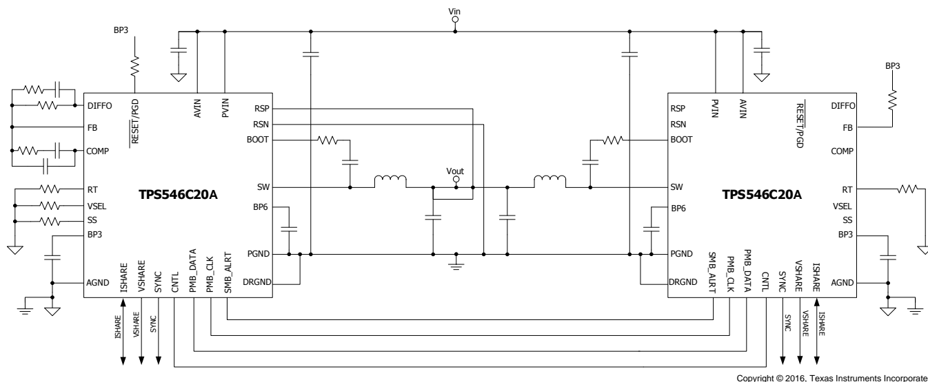
Figure 23. 2-Phase Application
