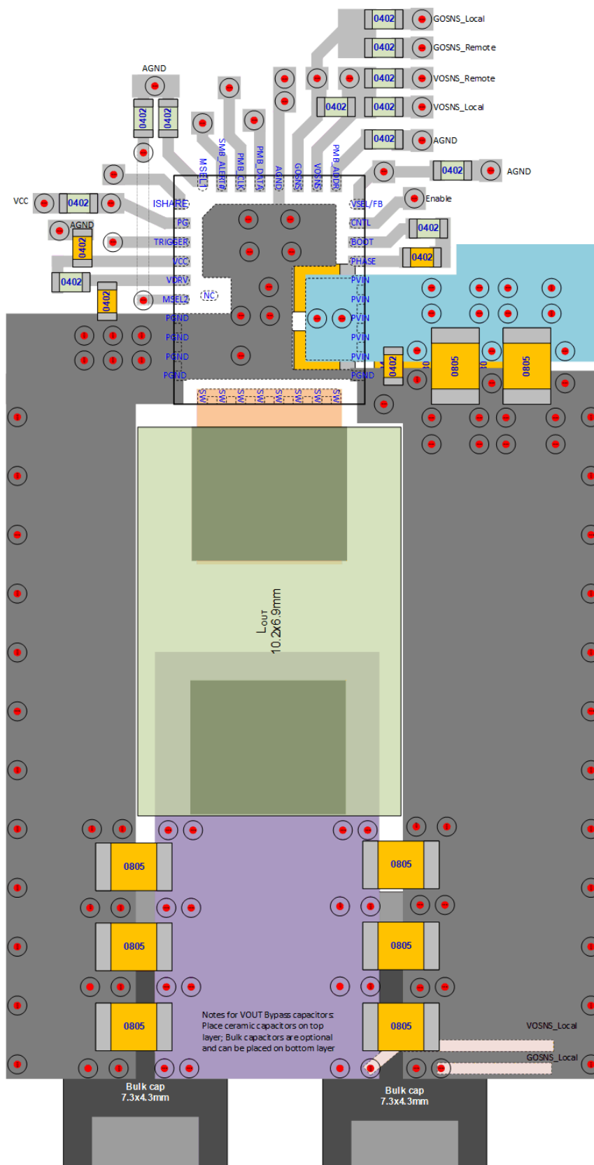
図 8-8. Layout Recommendation
