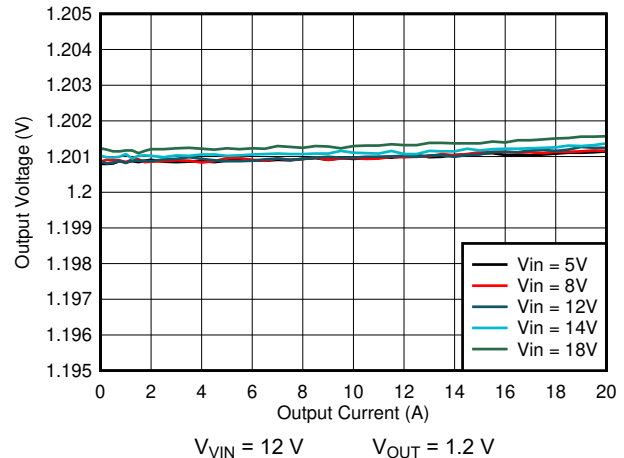
8-3. Load Regulation
