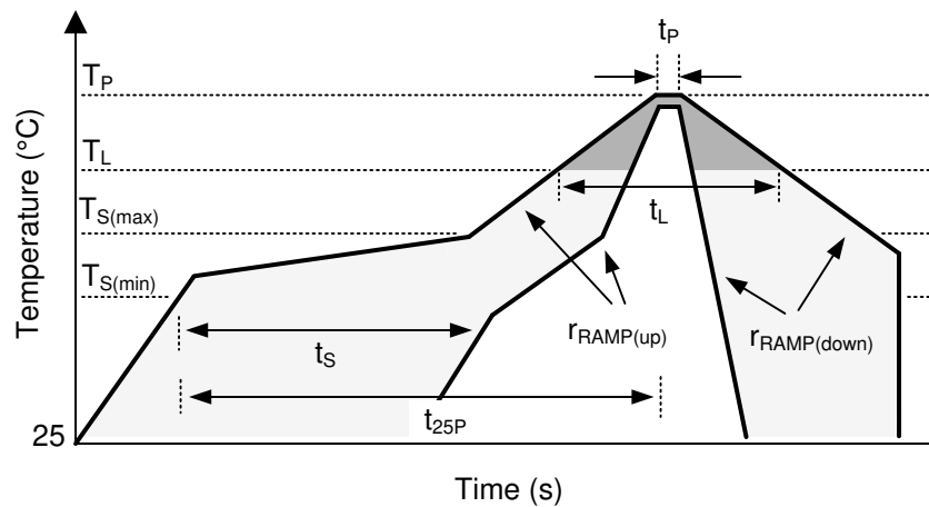
図 7-10. Recommended Reflow-Oven Thermal Profile
