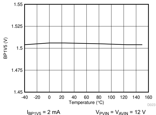
図 5-12. BP1V5 Voltage vs Junction Temperature
