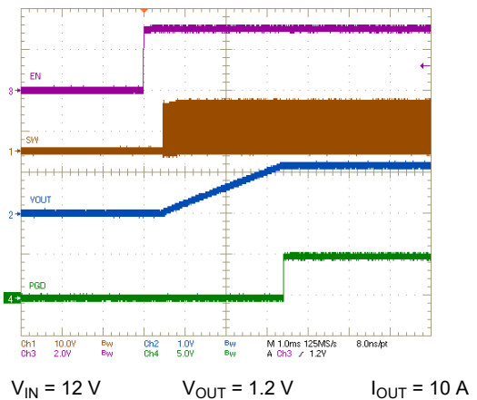
図 7-5. Start-Up from EN/UVLO
