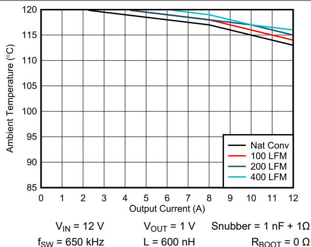
図 5-1. TPS546A24S Safe Operating Area
