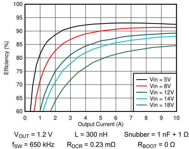
図 7-2. Efficiency vs Output Current
