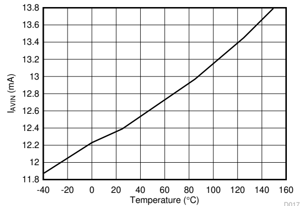
図 5-10. Non-Switching Input Current ( I_{AVIN} ) vs Junction Temperature
