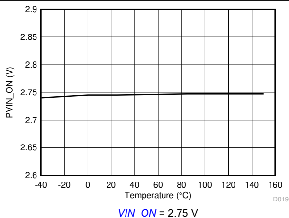
図 5-13. Turnon Voltage vs Junction Temperature
