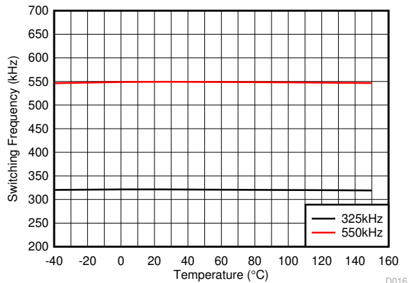
図 5-9. Switching Frequency vs Junction Temperature
