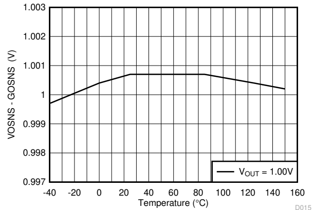
図 5-8. Output Voltage vs Junction Temperature
