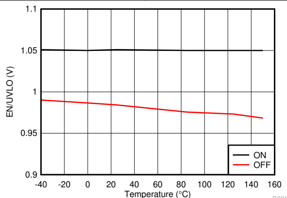
図 5-15. EN/UVLO Thresholds vs Junction Temperature
