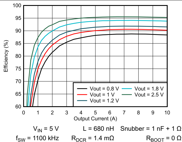
図 5-3. TPS546A24S Efficiency vs Output Current
