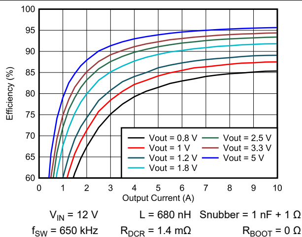
図 5-4. TPS546A24S Efficiency vs Output Current
