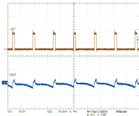
図 7-8. V_{OUT} Steady-State Ripple
