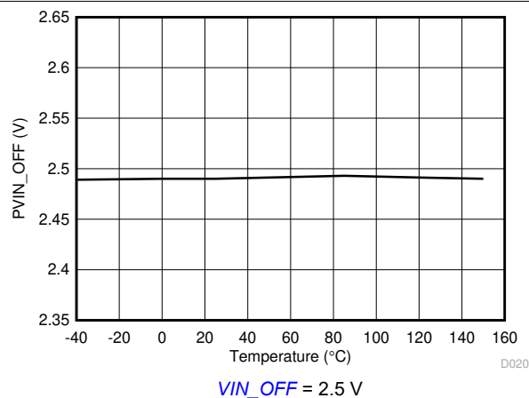
図 5-14. Turnoff Voltage vs Junction Temperature
