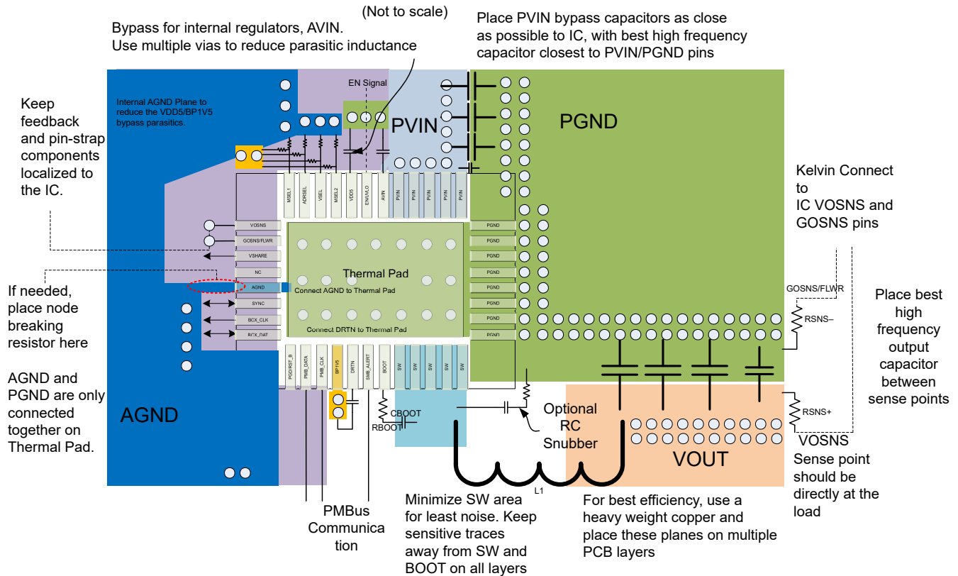
図 7-9. PCB Layout Recommendation
