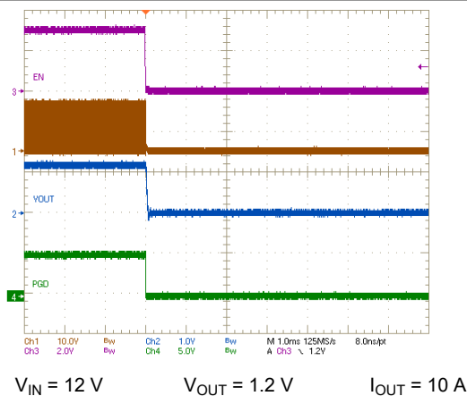
図 7-6. Shutdown from CNTL
