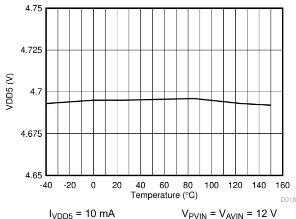
図 5-11. VDD5 Voltage vs Junction Temperature
