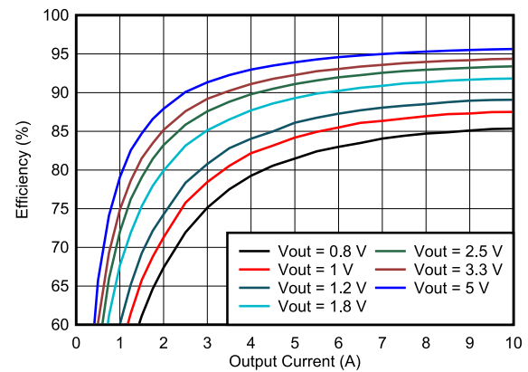
FIG 6-4. TPS546A24A Efficiency vs Output Current
