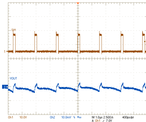
8-8. V_{OUT} Steady-State Ripple
