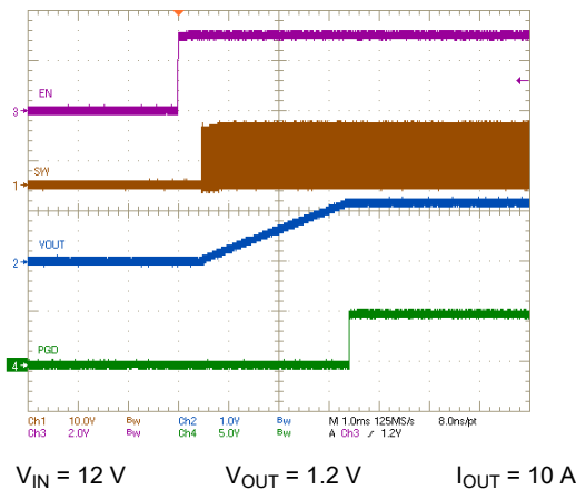
图 8-5. Start-Up from EN/UVLO
