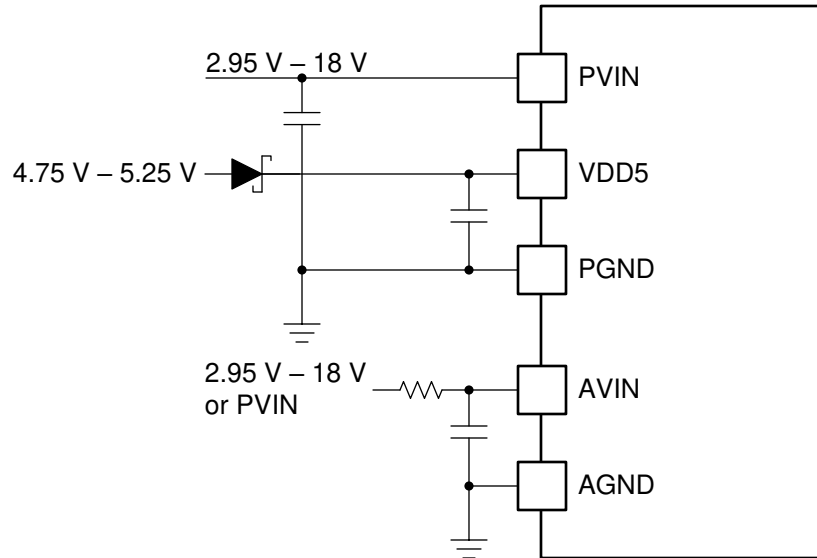
FIG 7-4. TPS546A24A Separate PVIN, AVIN, and VDD5 Connections
