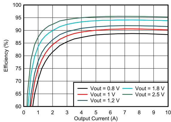
FIG 6-3. TPS546A24A Efficiency vs Output Current
