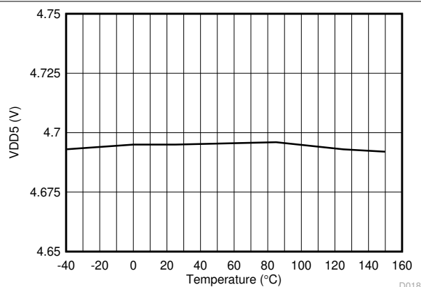
Figure 6-11. VDD5 Voltage vs Junction Temperature
