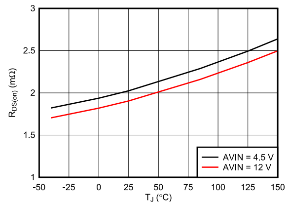
FIG 6-6. Low-Side MOSFET On-Resistance ( R_{DS(on)} ) vs Junction Temperature
