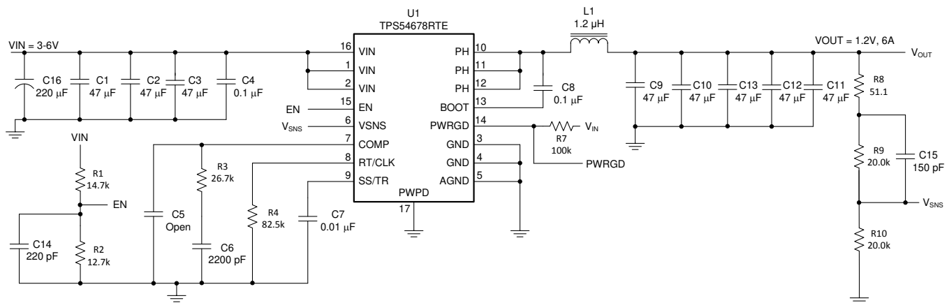
Figure 30. Typical Application Schematic, TPS54678
