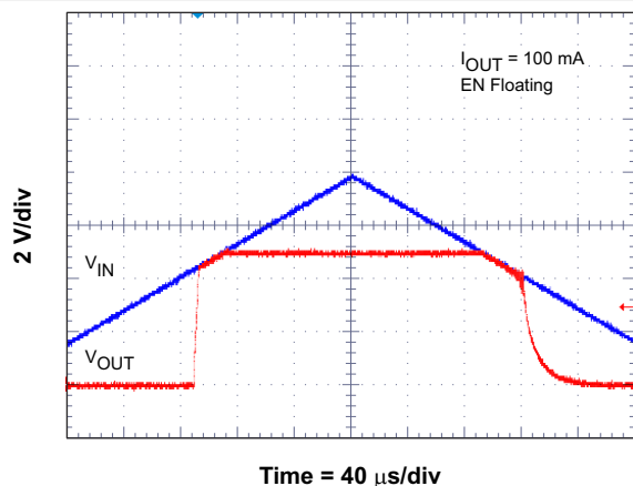
8-16. Low Dropout Operation
