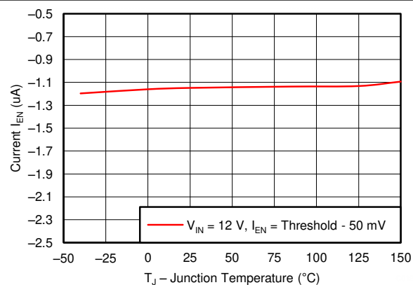
6-12. EN Pin Current vs Junction Temperature
