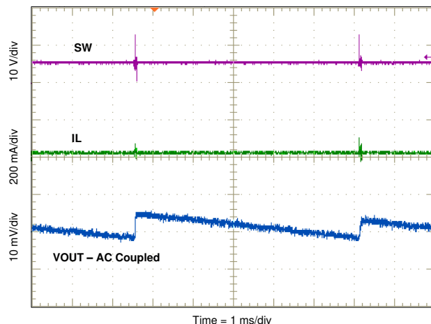
8-12. Output Ripple PSM
