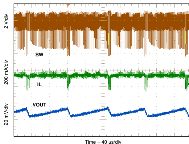
8-15. Low Dropout Operation
