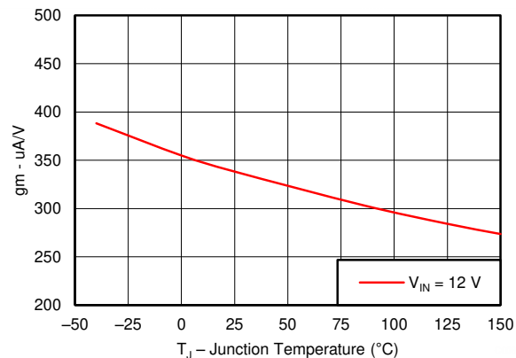
6-8. EA Transconductance vs Junction Temperature
