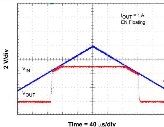
8-17. Low Dropout Operation
