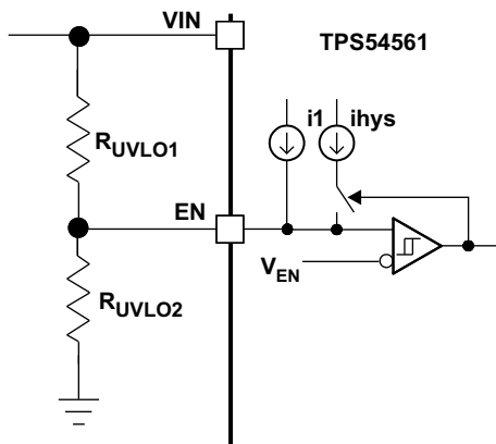
7-1. Adjustable Undervoltage Lockout (UVLO)
