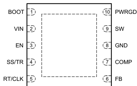
図 5-1. DPR Package 10-Pin WSON Top View
