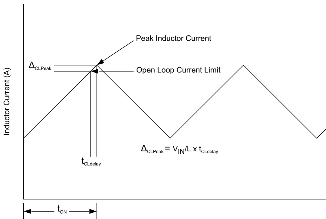
7-16. Current Limit Delay
