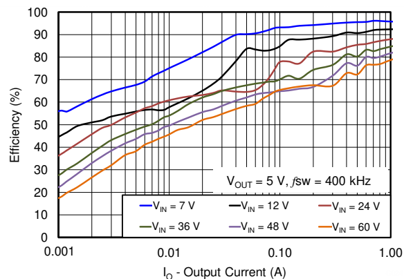
8-19. Light Load Efficiency
