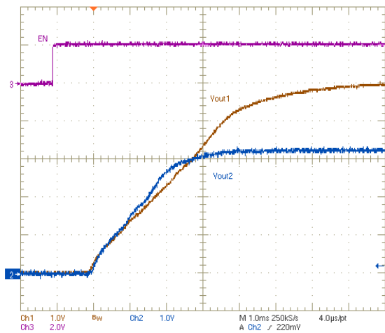
7-9. Ratio-Metric Startup with Tracking Resistors
