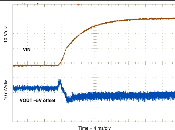
8-7. Line Transient (8 V to 40 V)
