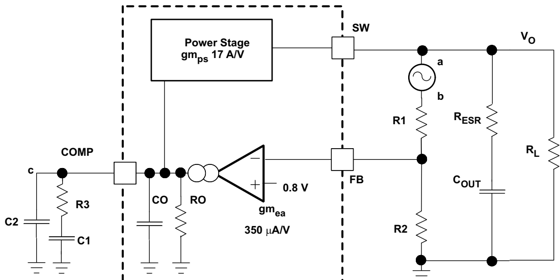
Figure 7-17. Small Signal Model for Loop Response
