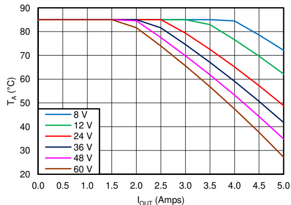
8-3. 5-V Output with 400-kHz Switching Frequency
