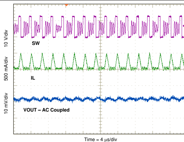
8-11. Output Ripple DCM
