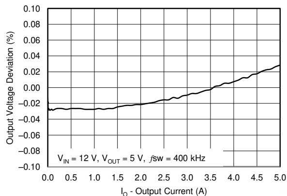
8-24. Regulation vs Load Current
