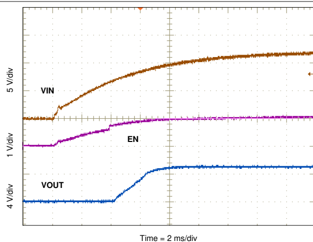
8-8. Start-up With VIN
