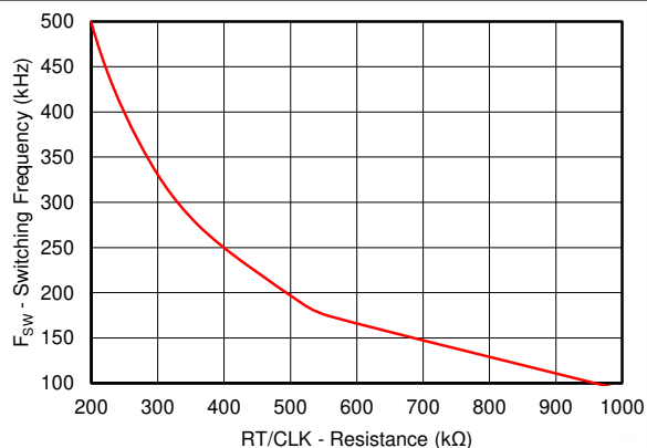
Figure 6-6. Switching Frequency vs RT/CLK Resistance Low Frequency Range
