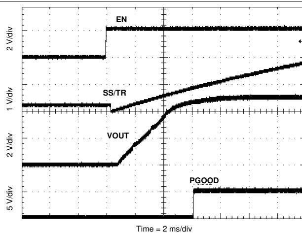
8-9. Start-up With EN
