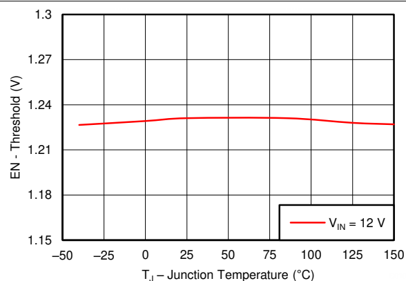
6-10. EN Pin Voltage vs Junction Temperature
