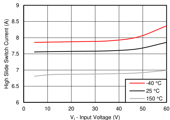
Figure 6-4. Switch Current Limit vs Input Voltage
