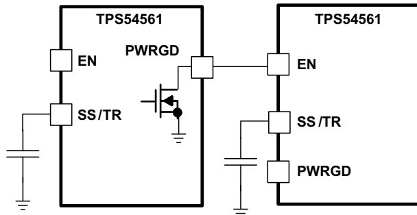
Figure 7-4. Schematic for Sequential Start-Up Sequence
