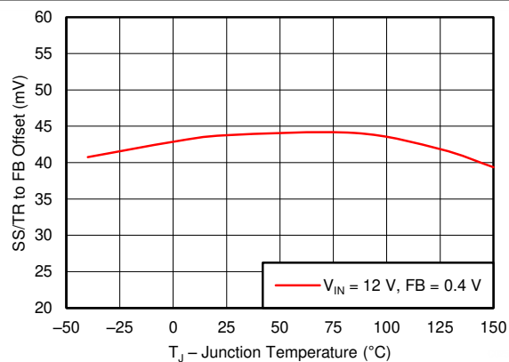
6-24. SS/TR to FB Offset vs Temperature
