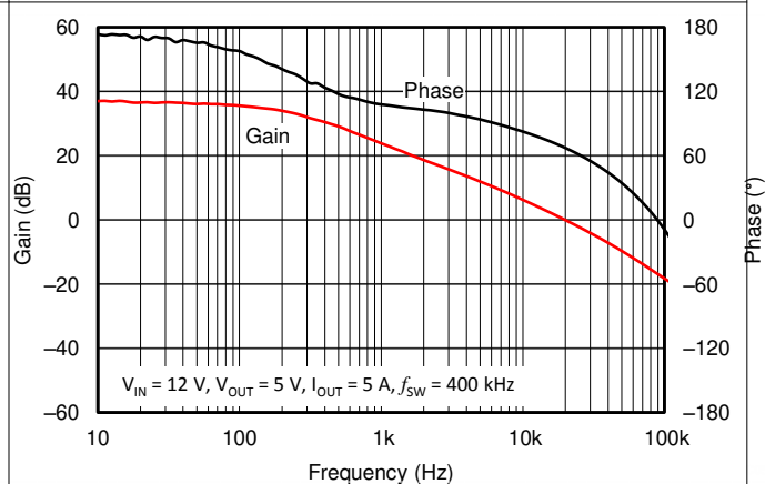
8-23. Overall Loop Frequency Response
