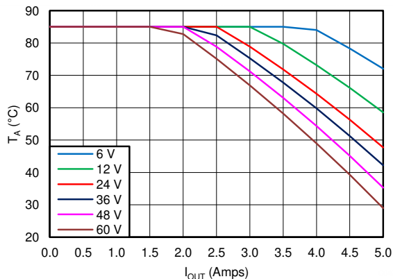
8-2. 3.3-V Output with 400-kHz Switching Frequency
