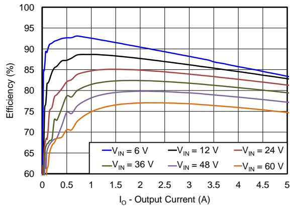
Figure 51. Efficiency vs Load Current
