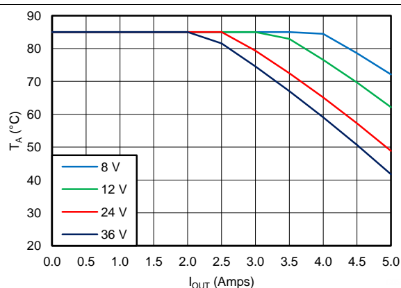
Figure 48. 5-V Outputs
