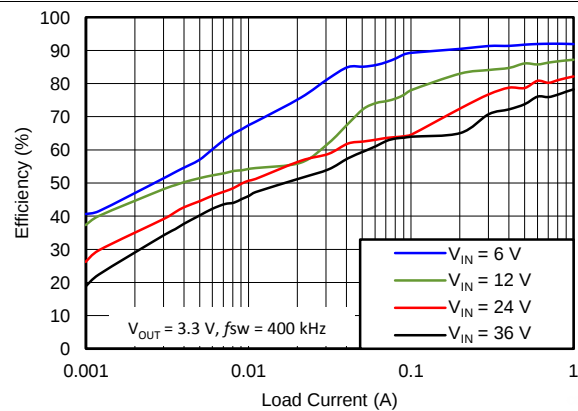
Figure 47. Light Load Efficiency
