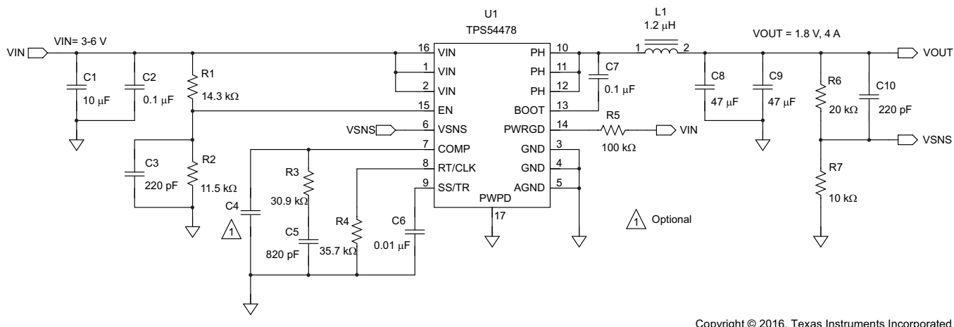
Figure 36. High Frequency, 1.8 V Output Power Supply Design with Adjusted UVLO
