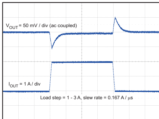
Figure 40. Transient Response, 2 A Step
