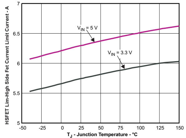
Figure 8. High Side FET Current Limit vs Temperature
