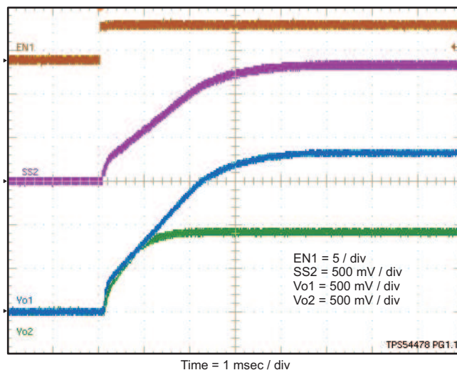
Figure 28. Simultaneous Start-Up using Coupled SS/TR Pins
