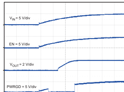
Figure 41. Power Up VOUT, VIN
