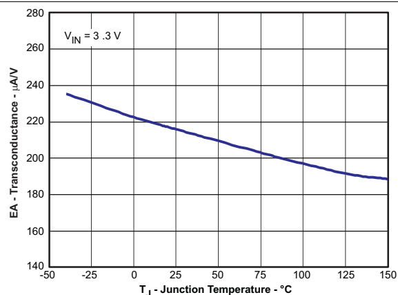
Figure 8. Transconductance vs Junction Temperature
