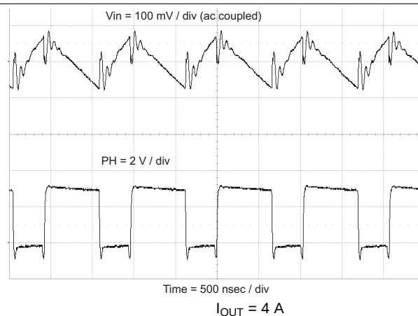
Figure 49. Input Ripple
