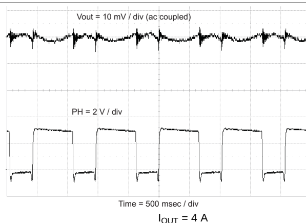
Figure 47. Output Ripple
