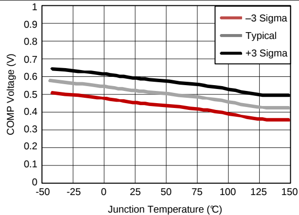
Figure 22. Comp Voltage Clamp vs Junction Temperature
