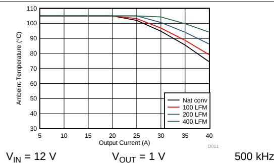
⊠ 45. Safe Operating Area
