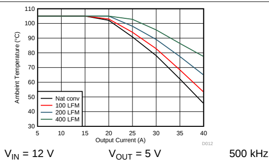
⊠ 44. Safe Operating Area
