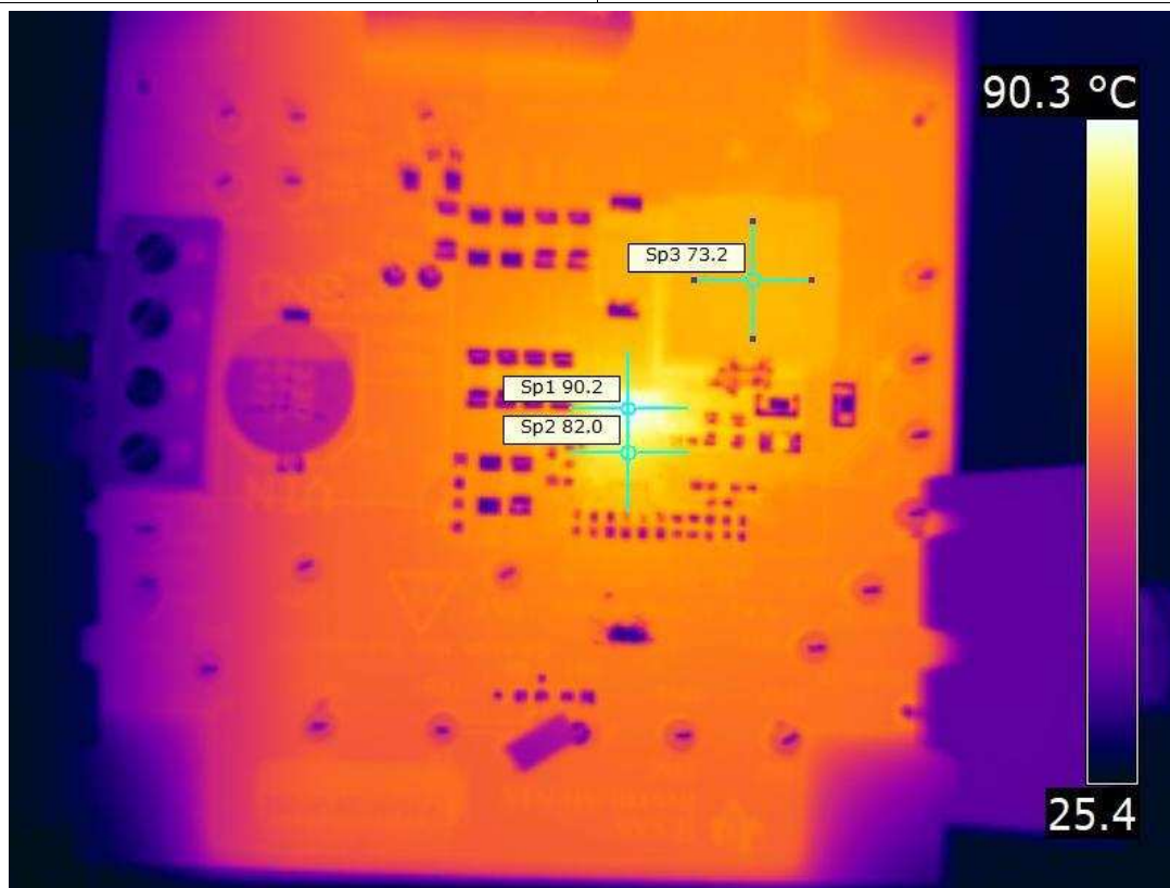
⊠ 46. Thermal Image at 1.0-V Output at 12 V_{IN} , 40-A Output, at 25°C Ambient
