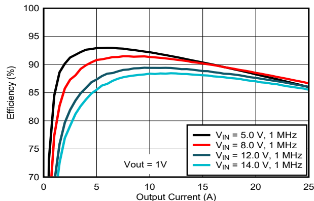
図 7-4. Efficiency Curves
