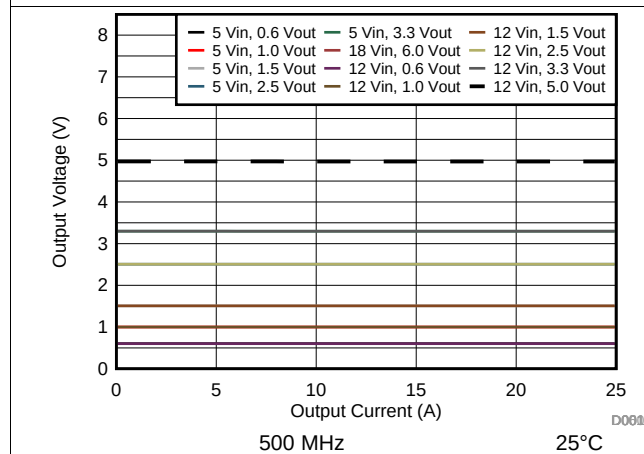
FIG 5. Output Current vs Output Voltage
