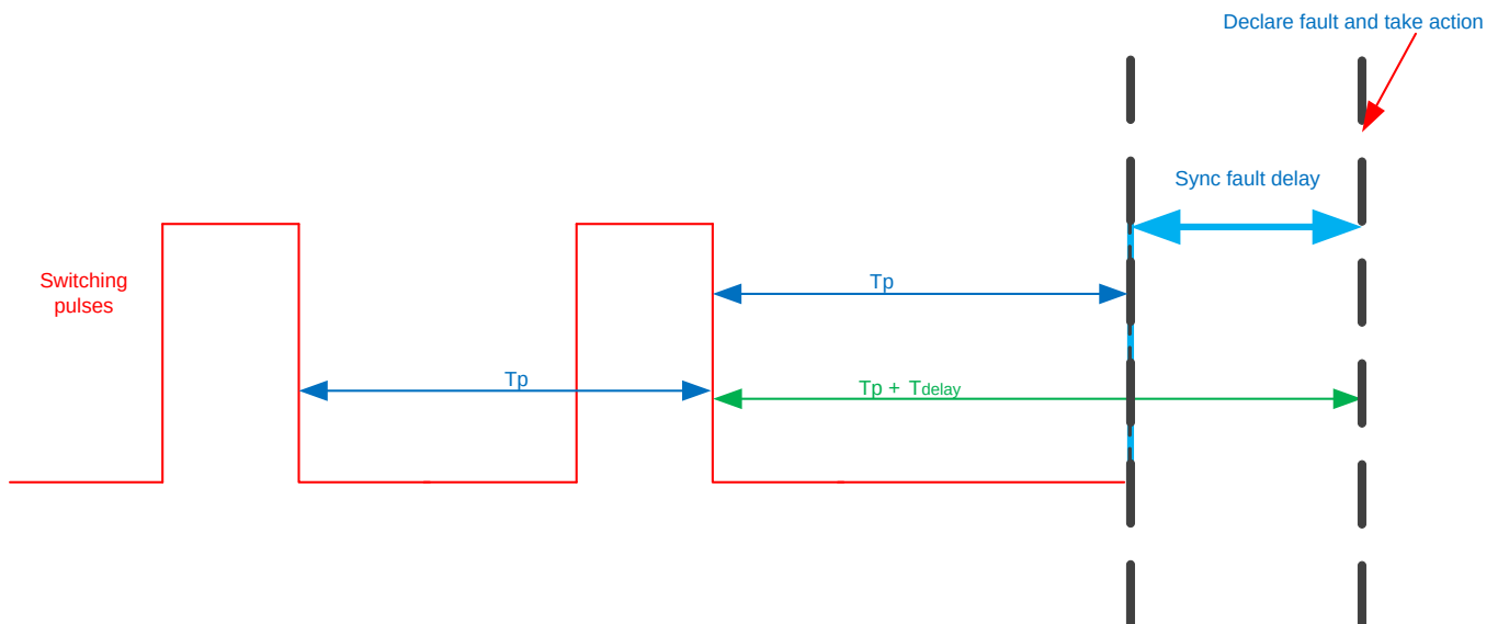
23. Switching Response When Sync Clock Lost
