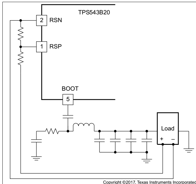
21. Remote Sensing With Feedback Resistors
