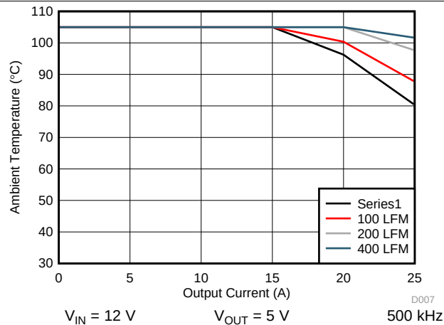
Figure 39. Safe Operating Area
