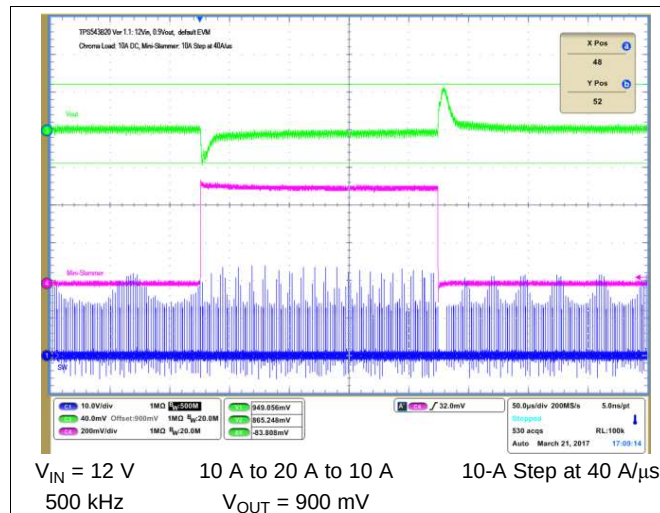
FIG 7. Output Voltage Transient Response
