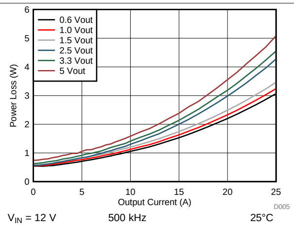
FIG 4. Power Loss vs Output Current
