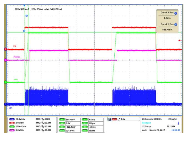
12. Output Voltage Start-Up and Shutdown
