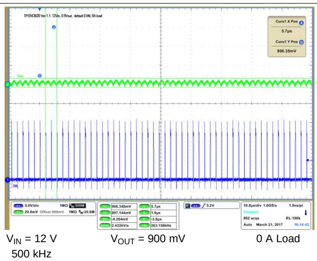
FIG 8. Output Voltage Ripple at Steady State
