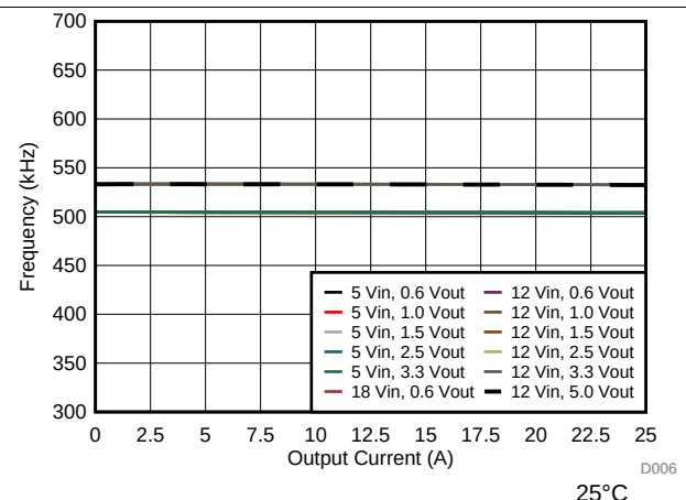
FIG 6. Switching Frequency vs Output Current
