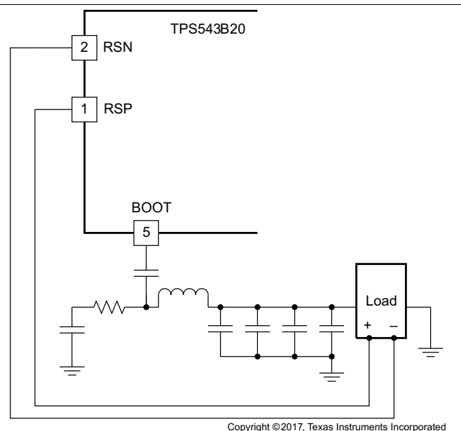
22. Remote Sensing Without Feedback Resistors
