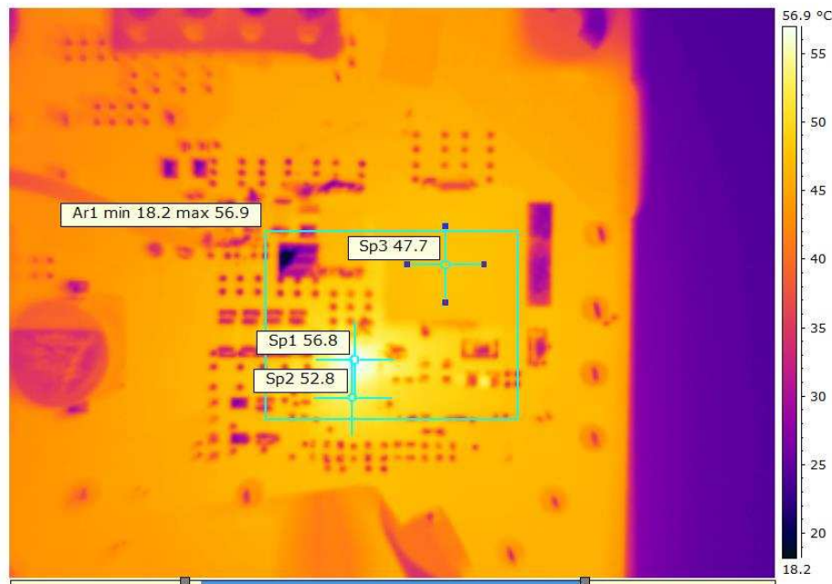
Figure 41. Thermal Image at 0.9-V Output at 12 VIN, 25-A Output, at 25°C Ambient
