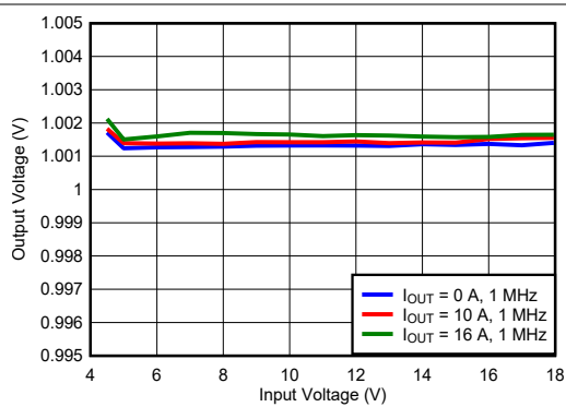
Figure 7-6. Line Regulation
