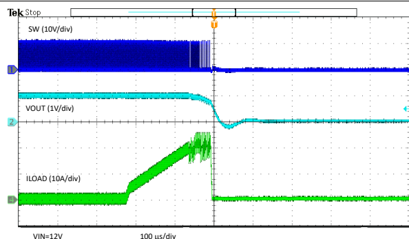
7-20. Overcurrent Protection – Overload
