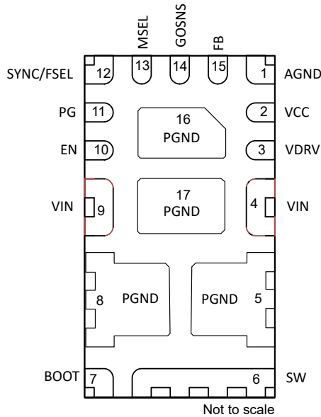
図 4-1. 17-Pin WQFN-FCRLF RYS Package (Bottom View)
