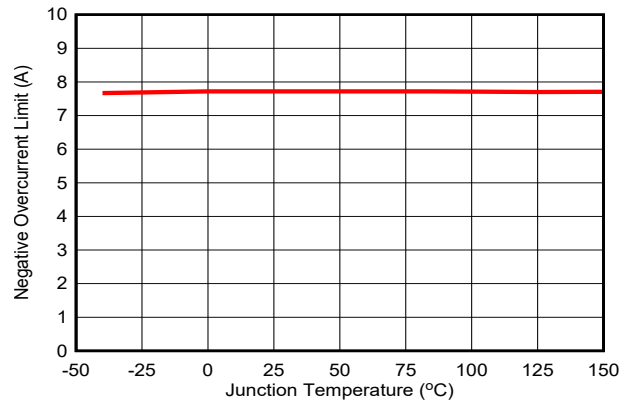
図 5-4. Negative Overcurrent Limit
