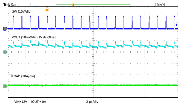
7-16. Output Ripple – No Load
