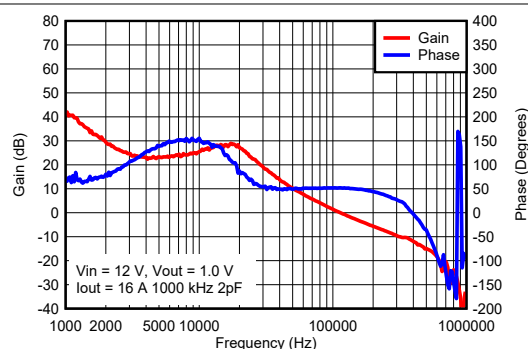
Figure 7-7. Bode Plot
