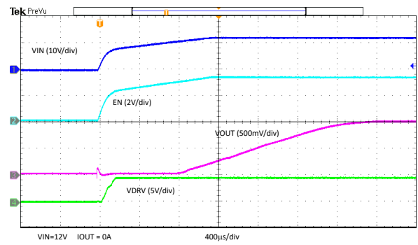
図 7-9. EN Start-up – Measuring BP5
