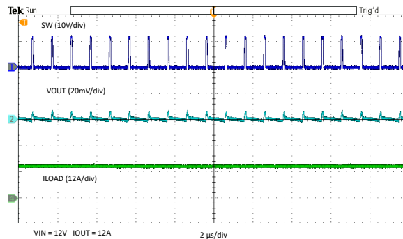
7-17. Output Ripple – Full Load
