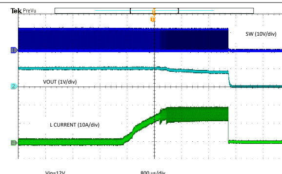
7-21. Overcurrent Protection – Short
