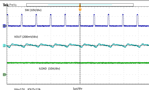
7-17. Output Ripple – Full Load
