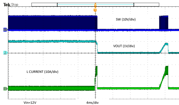
図 7-22. Overcurrent Protection – Hiccup and Recover
