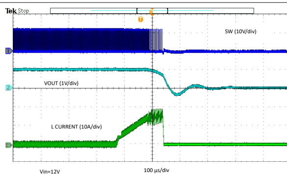
7-20. Overcurrent Protection – Overload
