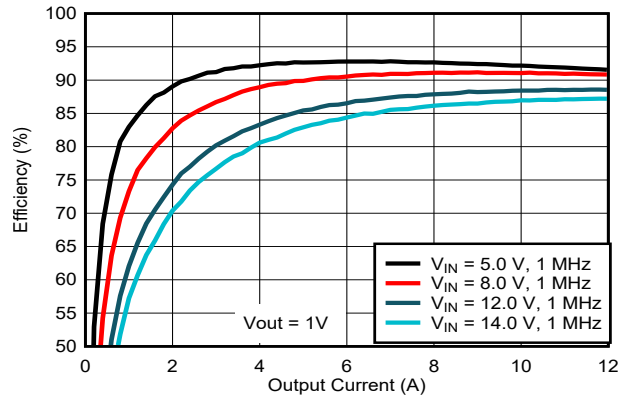
図 7-4. Efficiency Curves
