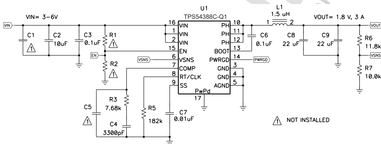
図 8-1. High-Frequency, 1.8-V Output Power-Supply Design With Adjusted UVLO
