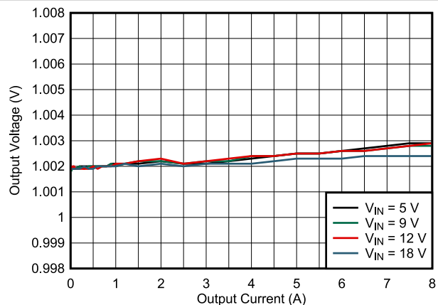
Figure 8-5. Load Regulation
