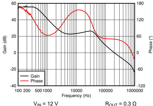
Figure 8-27. Bode Plot
