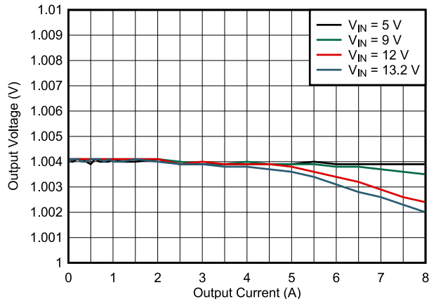
Figure 8-26. Load Regulation
