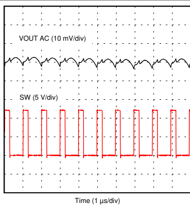
8-35. Output Ripple – No Load
