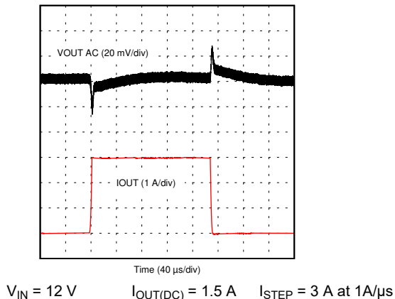
Figure 8-25. Load Transient
