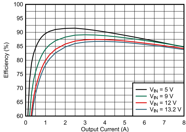
Figure 8-24. Efficiency
