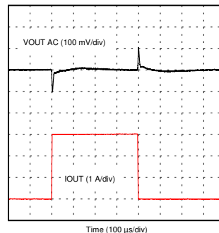
8-32. Load Transient
