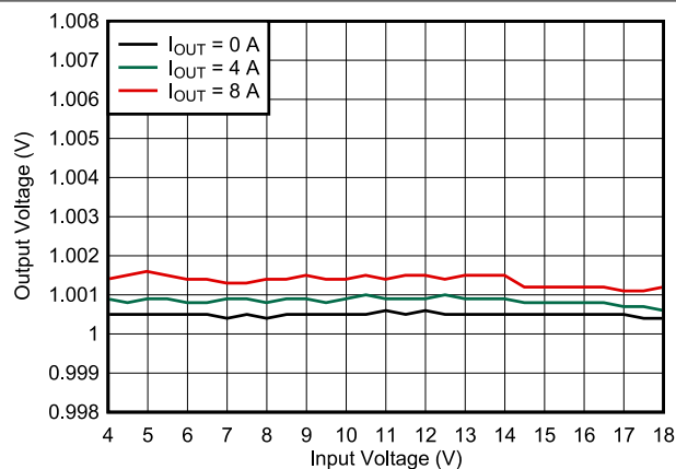
Figure 8-6. Line Regulation
