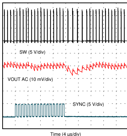
7-4. Clock Synchronization Transitions
