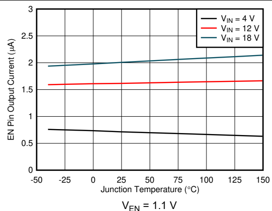
Figure 6-10. EN Pin Current vs Junction Temperature
