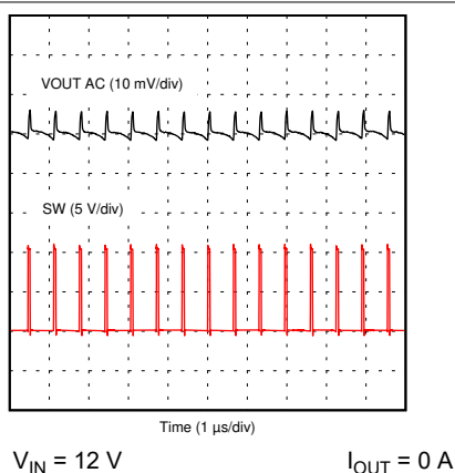
Figure 8-28. Output Ripple – No Load
