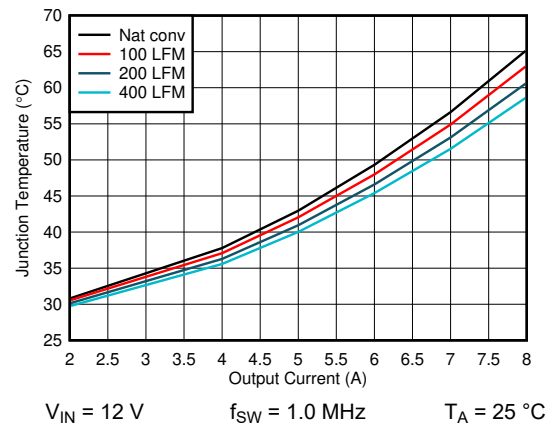
Figure 6-8. Junction Temperature vs Output Current – 3.3-V Output
