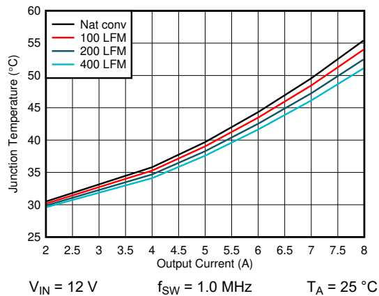
Figure 6-7. Junction Temperature vs Output Current – 1-V Output
