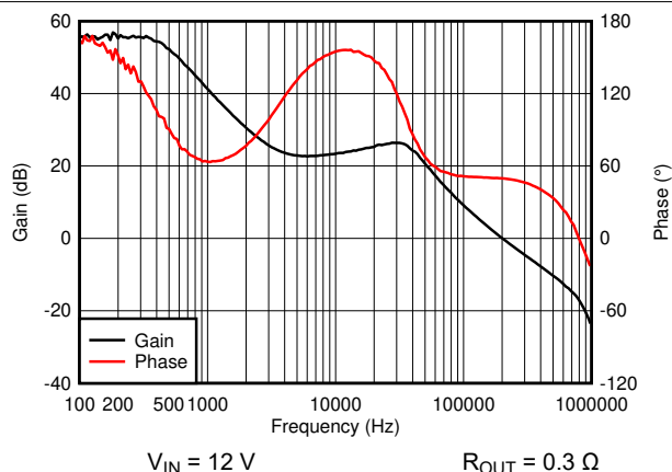
Figure 8-27. Bode Plot
