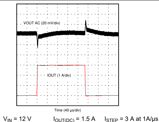
Figure 8-25. Load Transient
