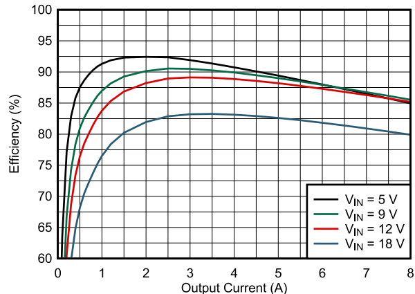
Figure 8-4. Efficiency
