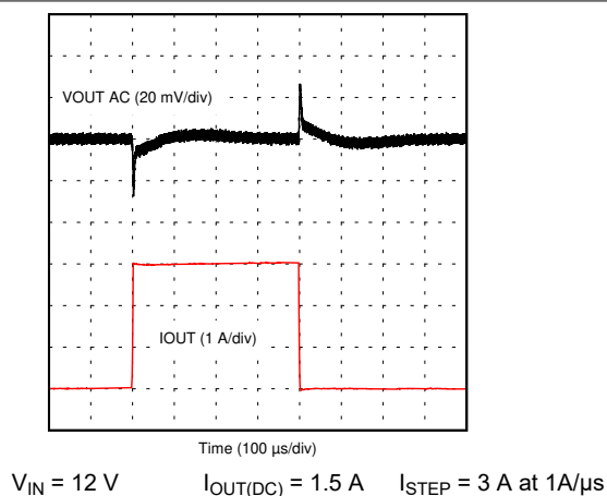
Figure 8-8. Load Transient
