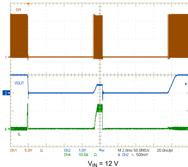
8-22. Overcurrent Protection – Hiccup and Recover
