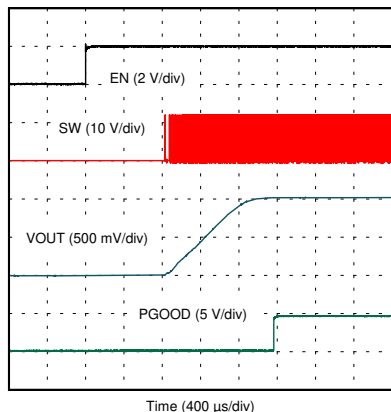
8-10. EN Startup – Measuring SW
