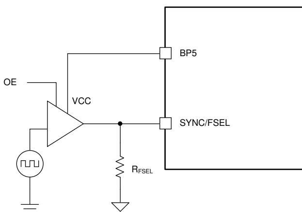
7-5. Interfacing the SYNC/FSEL Pin with a Buffer
