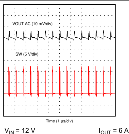
Figure 8-29. Output Ripple – 6-A Load
