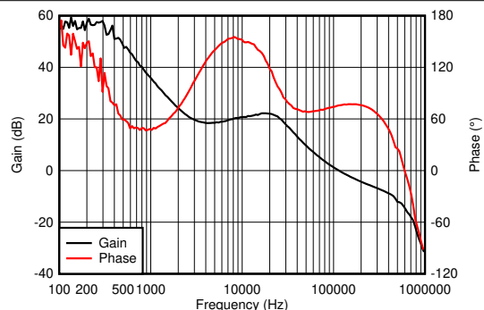
8-34. Bode Plot
