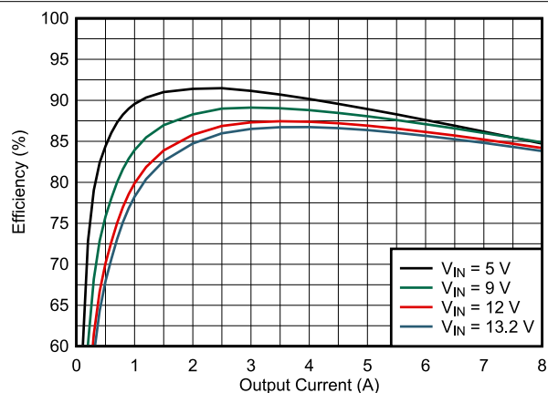
Figure 8-24. Efficiency
