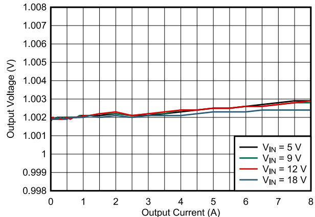
Figure 8-5. Load Regulation
