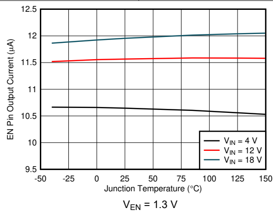
Figure 6-11. EN Pin Current vs Junction Temperature
