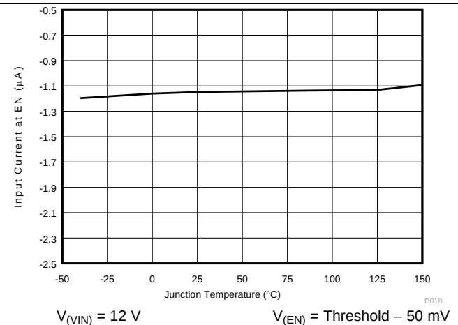
Figure 12. EN Pin Current vs Junction Temperature
