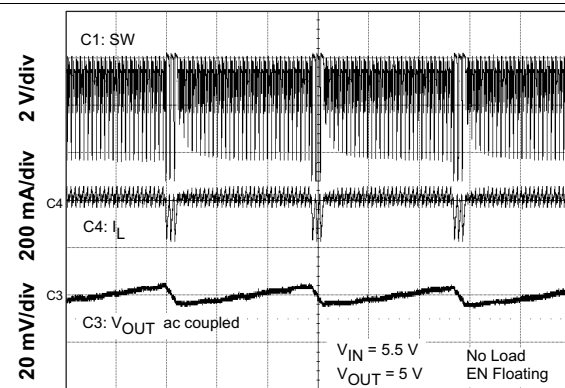
Time = 20 μs/div Figure 43. Low Dropout Operation
