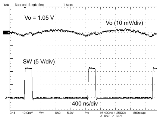
Figure 12. VOLTAGE RIPPLE AT OUTPUT ( I_O = 3\text{ A} )
