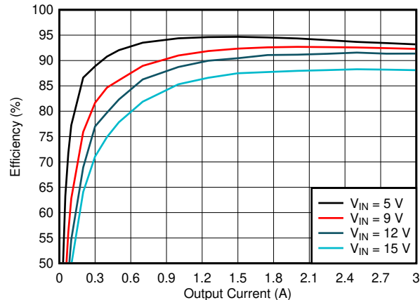
8-22. Efficiency
