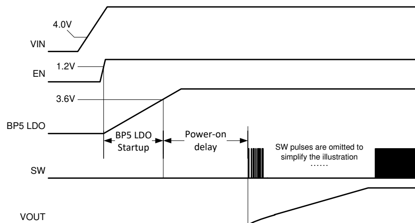
図 7-1. Start-Up Sequence
