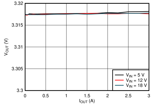
图 8-5. Load Regulation
