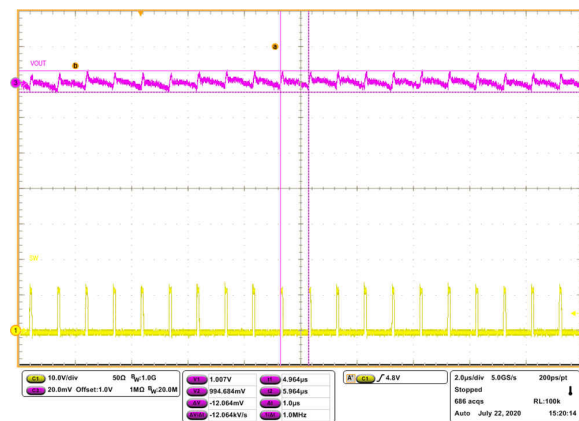
図 6-20. Steady State at 0-A Output Current
