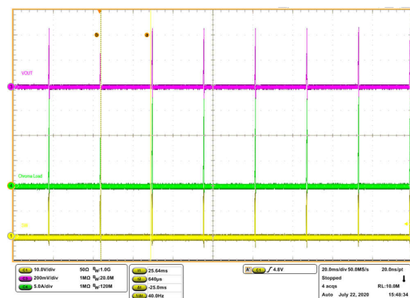
図 6-22. Switch Node Ringing and Dead-Time at 10-A Output Current
