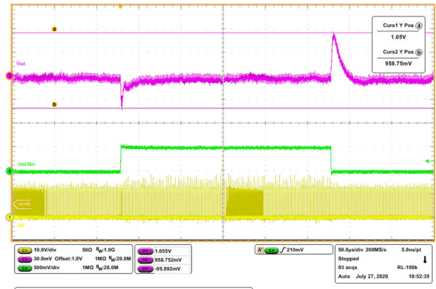
6-26. Load Transient 2 A to 12 A to 2 A at 20 A/ \mu s
