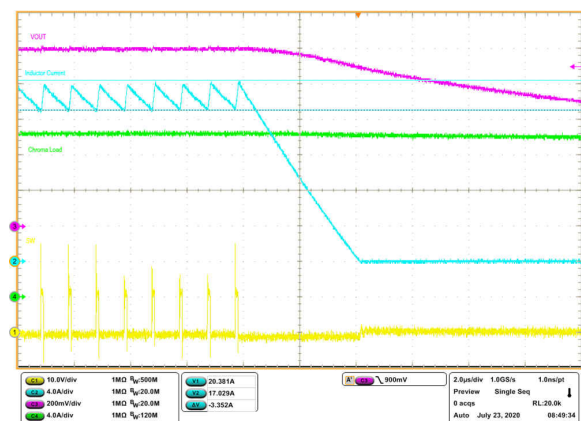
図 6-23. 20-A Overcurrent Protection by Chroma Electronic Load
