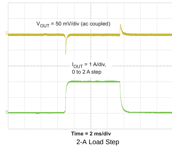
Figure 41. Transient Response
