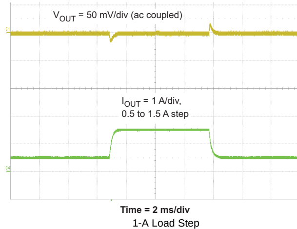
Figure 40. Transient Response
