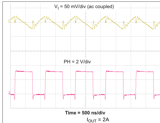
Figure 50. Input Ripple
