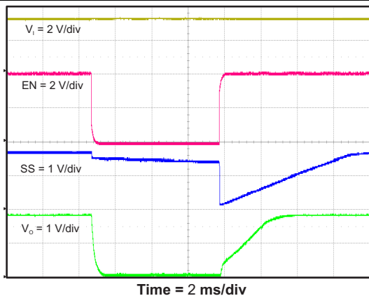
Figure 46. SS Discharge During EN Disable / Enable
