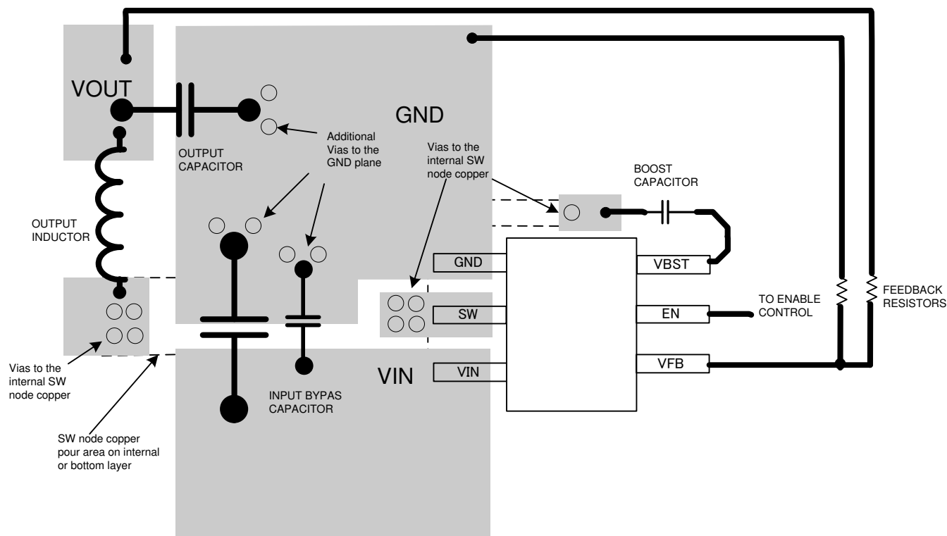
10-1. Board Layout
