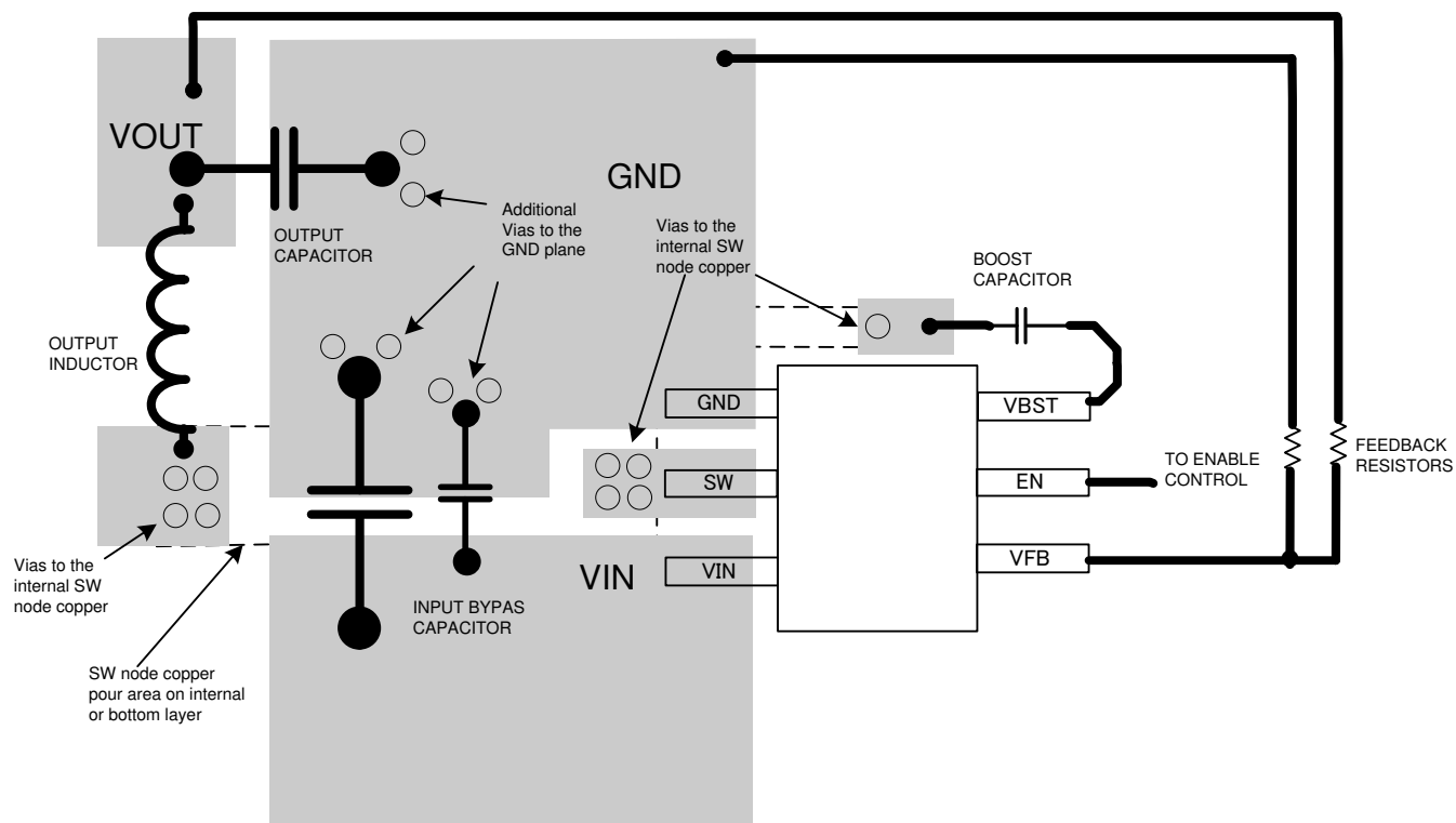
10-1. Board Layout
