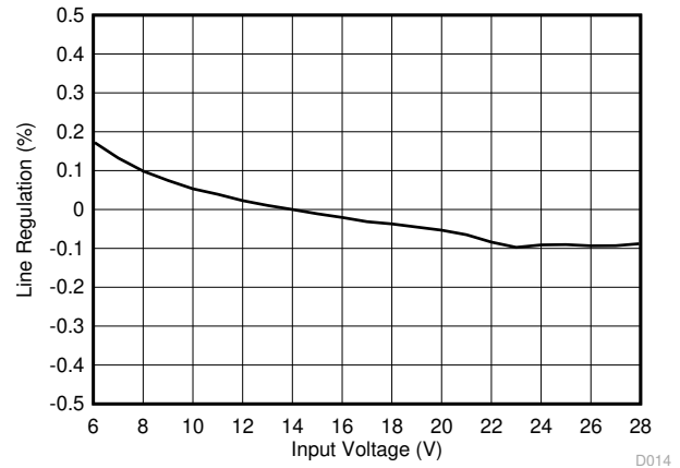
图 8-3. Line Regulation
