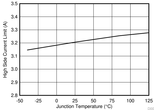
FIG 6-7. High-Side Current Limit Threshold vs Junction Temperature
