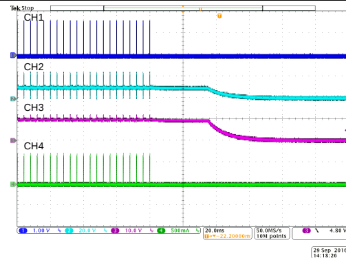
CH1: PWM CH2: SW CH3: V_{OUT} CH4: LED current
