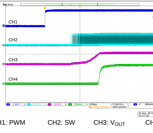
图 43. Start-Up at 100% PWM Duty Cycle
