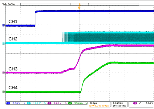
图 30. Start-Up at 1% PWM Duty Cycle and 50 kHz
