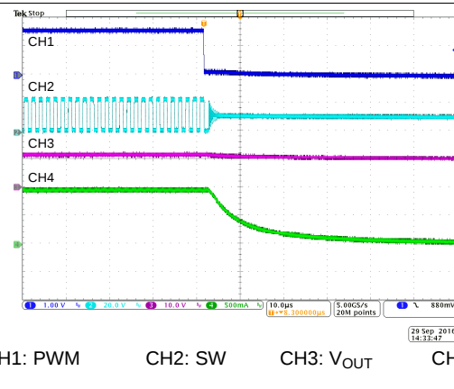
图 44. Shutdown at 100% PWM Duty Cycle
