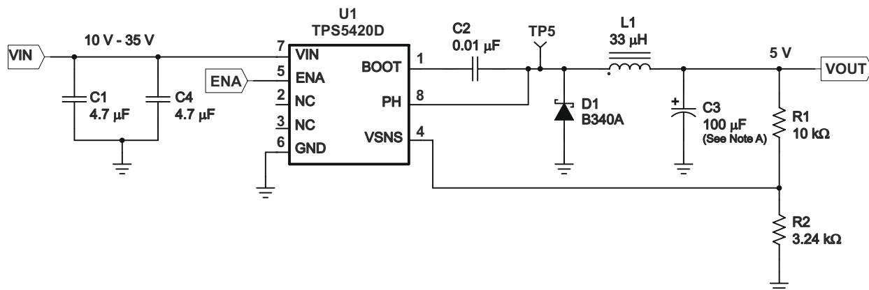
図 8-3. Application Circuit, 10-V — 35 V to 5-V
