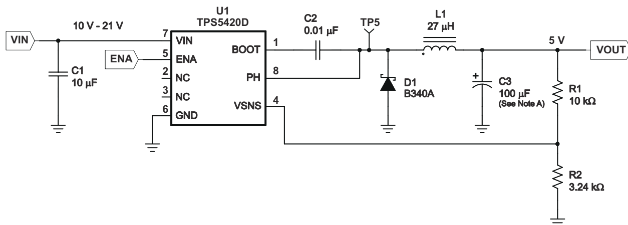
✎ 8-4. 10-V — 21-V Input to 5-V Output Application Circuit
