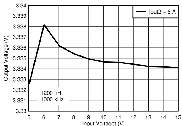
图 8-10. Line Regulation V_{OUT2}
