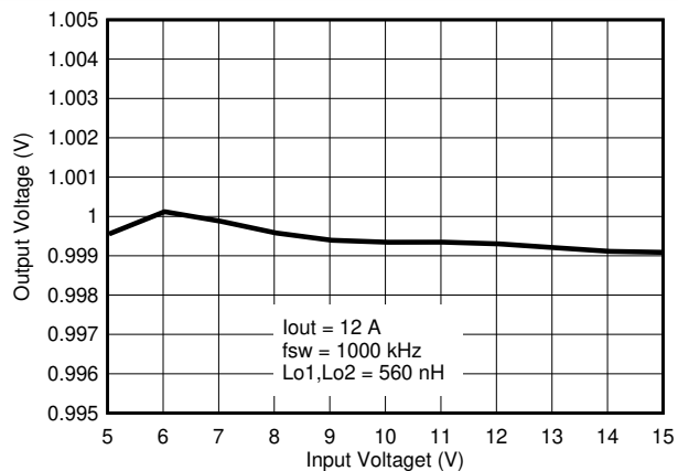
8-36. Line Regulation
