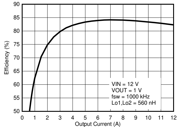
8-34. Efficiency
