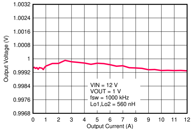
8-35. Load Regulation
