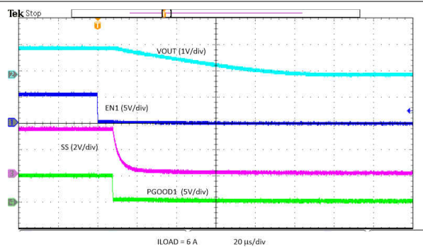
8-40. Power Down with EN
