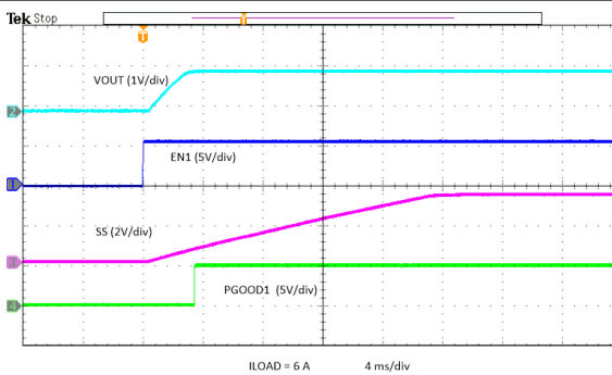
8-39. Power Up with EN
