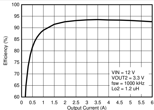
Figure 8-4. V OUT2 Efficiency
