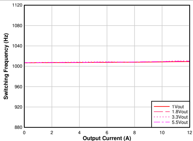
6-8. Switching Frequency vs Output Current, V_{IN} = 12\text{ V} , F_{SW} = 1\text{ MHz}
