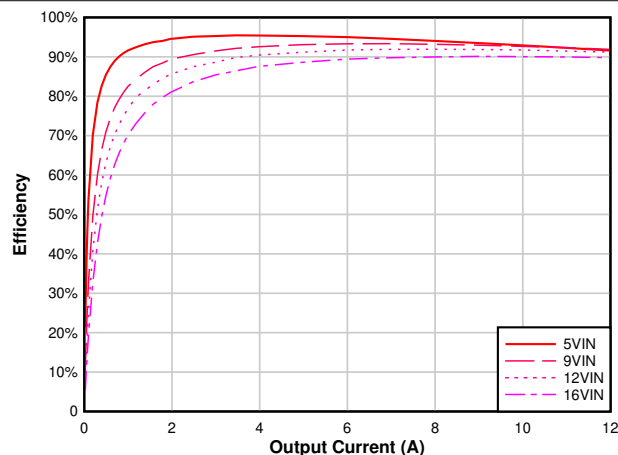
FIG 6-3. Efficiency vs Output Current, V_{OUT} = 3.3\text{ V} , F_{SW} = 1\text{ MHz}
