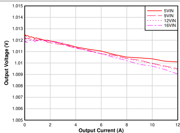
FIG 6-6. Output Voltage Regulation vs Output Current, V_{OUT} = 1.0\text{ V} , F_{SW} = 1\text{ MHz}
