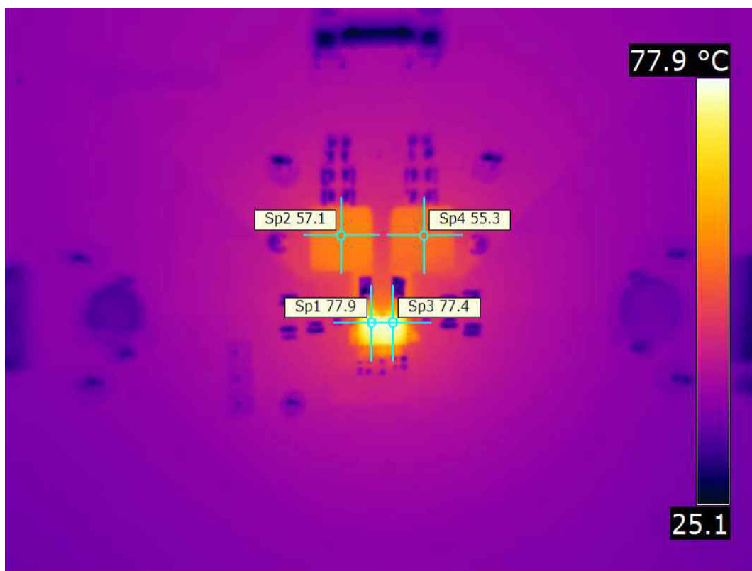
✎ 10-4. Thermal Image at 25°C Ambient - Dual Output Operation, f_{sw} = 1 \text{ MHz} , V_{IN} = 12 \text{ V} , V_{OUT1} = 1 \text{ V} , I_{OUT1} = 6 \text{ A} , L_1 = 560 \text{ nH} (3.3 mΩ Max), V_{OUT2} = 3.3 \text{ V} , I_{OUT2} = 6 \text{ A} , L_2 = 1.2 \text{ } \mu\text{H} (7.5 mΩ Max)
