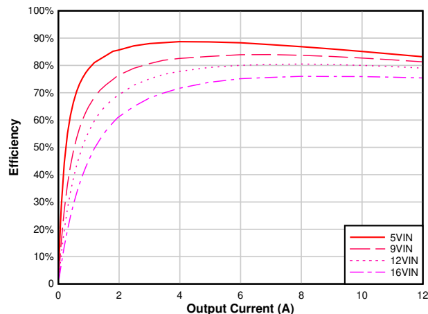
FIG 6-1. Efficiency vs Output Current, V_{OUT} = 1.0\text{ V} , F_{SW} = 1\text{ MHz}
