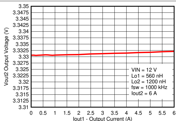
Figure 8-8. V OUT2 Cross Regulation
