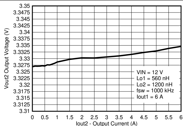
Figure 8-6. V OUT2 Load Regulation
