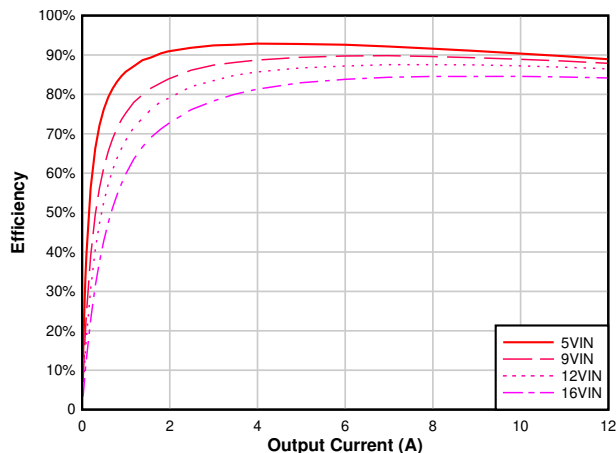
FIG 6-2. Efficiency vs Output Current, V_{OUT} = 1.8\text{ V} , F_{SW} = 1\text{ MHz}
