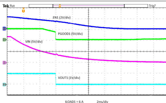
8-24. Power Down with V_{IN} V_{OUT1}
