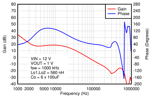
8-37. Bode Plot
