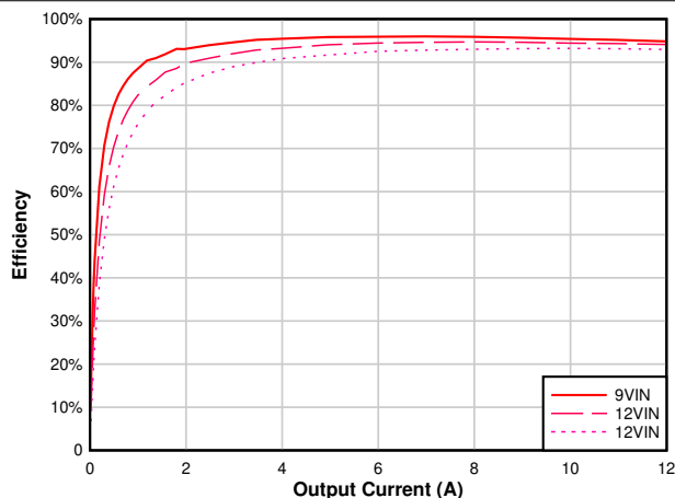
FIG 6-4. Efficiency vs Output Current, V_{OUT} = 5.5\text{ V} , F_{SW} = 1\text{ MHz}
