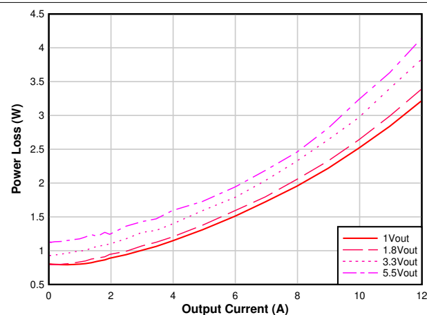
FIG 6-5. Power Dissipation vs Output Current, V_{IN} = 12\text{ V} , F_{SW} = 1\text{ MHz}
