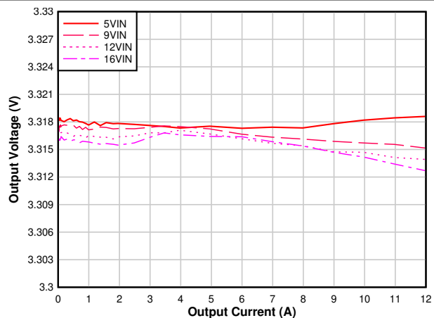
6-7. Output Voltage Regulation vs Output Current, V_{OUT} = 3.3\text{ V} , F_{SW} = 1\text{ MHz}
