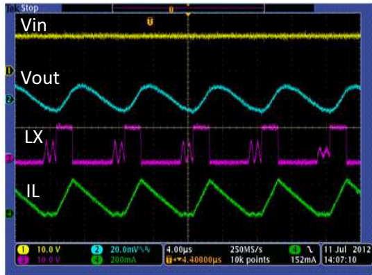
Figure 7. Steady State I_O = 100\text{ mA}
