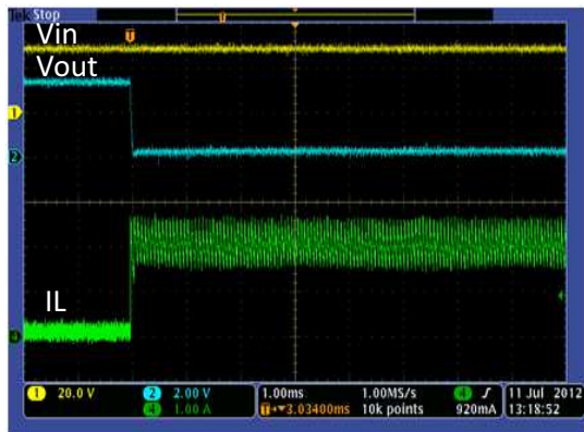
Figure 9. Short Circuit Protection
